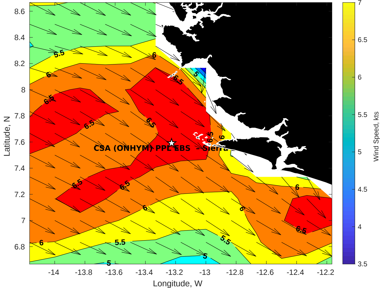
GFS Winds (kts) for CSA (ONHYM) PPL EBS - Sierra Leone at 29-Jan-2026 09:00:00
