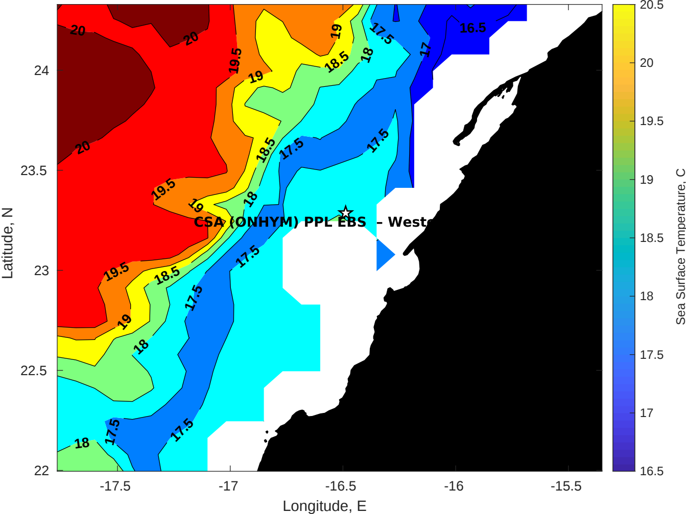
SST for CSA (ONHYM) PPL EBS - Western Sahara at 28-Jan-2026 00:00:00
