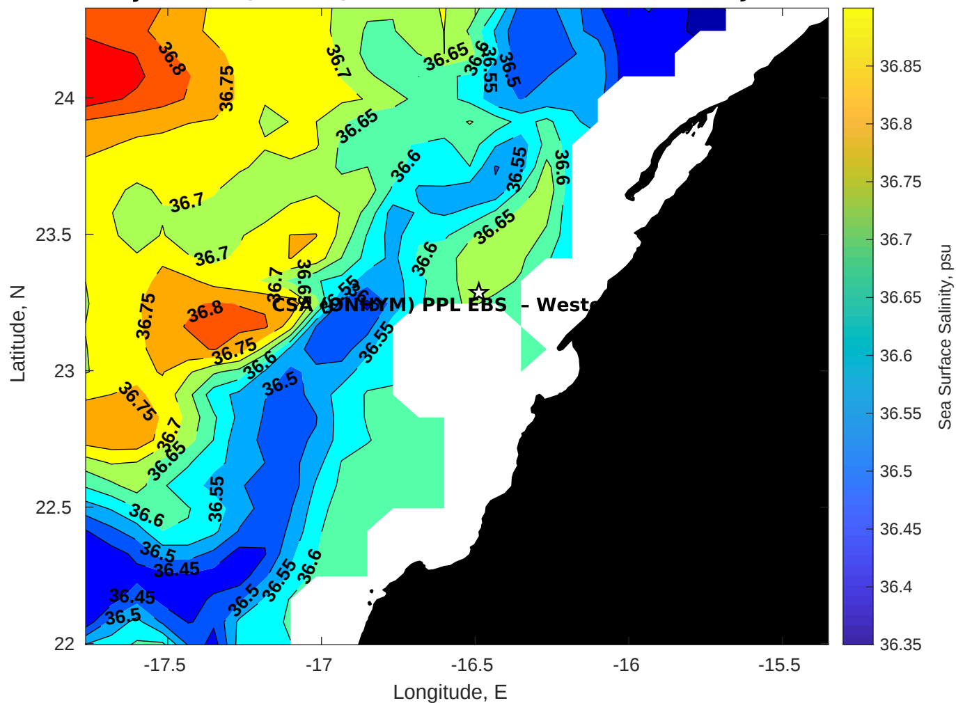
Surface Salinity for CSA (ONHYM) PPL EBS - Western Sahara at 28-Jan-2026 00:00:00
