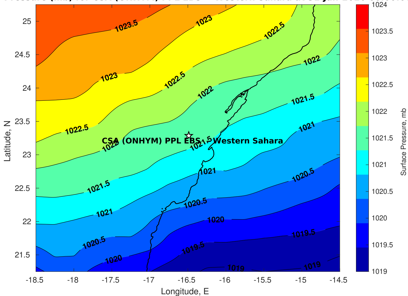
Surface Pressure (mb) for CSA (ONHYM) PPL EBS - Western Sahara at 31-Jan-2026 00:00:00
