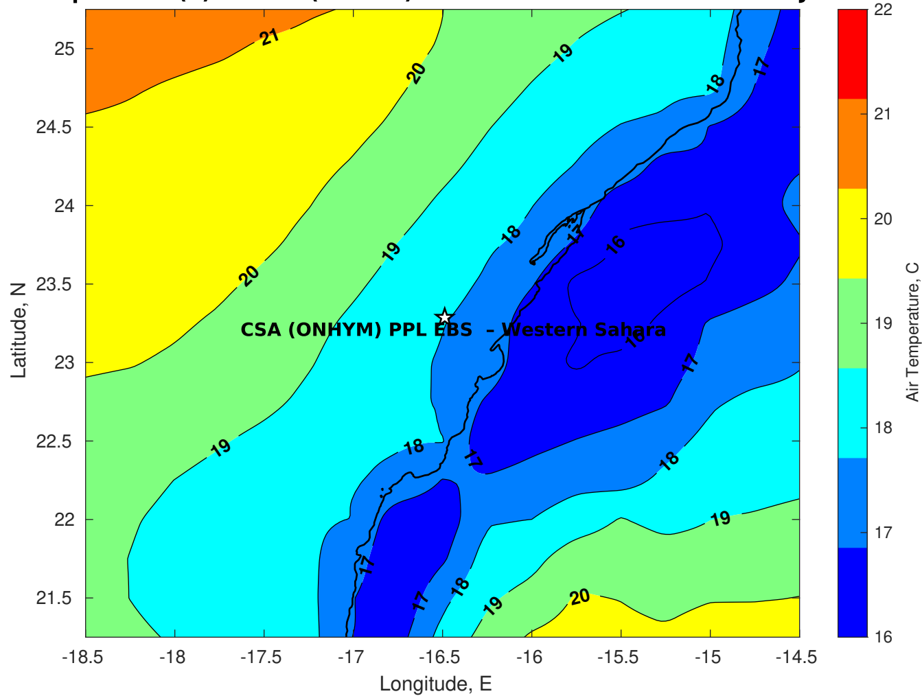
Air Temperature (C) for CSA (ONHYM) PPL EBS - Western Sahara at 29-Jan-2026
