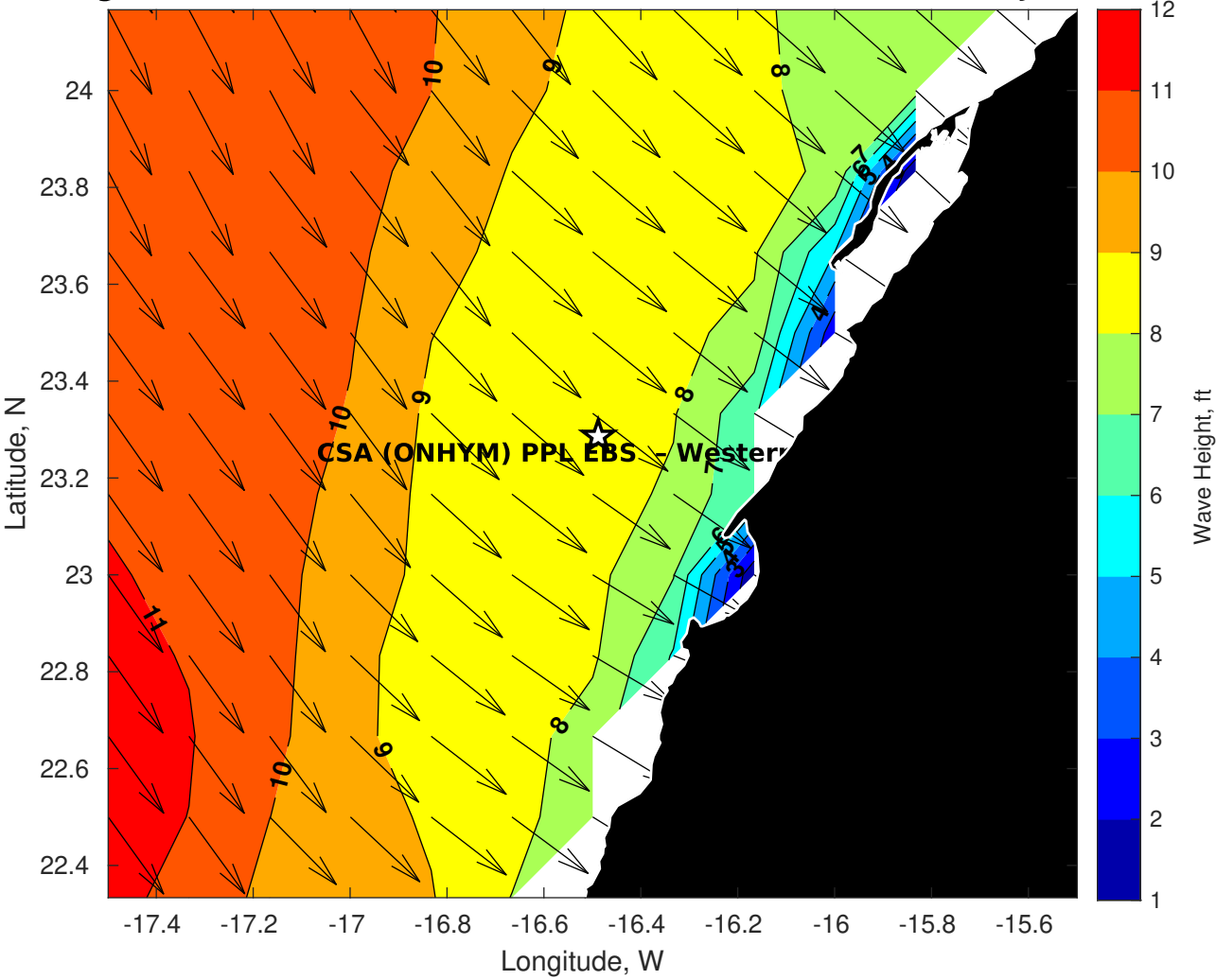
GFS Wave Height (ft) for CSA (ONHYM) PPL EBS - Western Sahara at 29-Jan-2026 09:00:00
