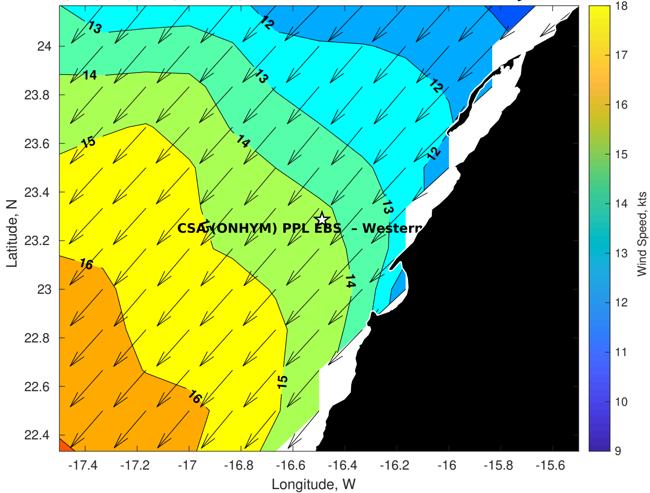
GFS Winds (kts) for CSA (ONHYM) PPL EBS - Western Sahara at 29-Jan-2026 09:00:00
