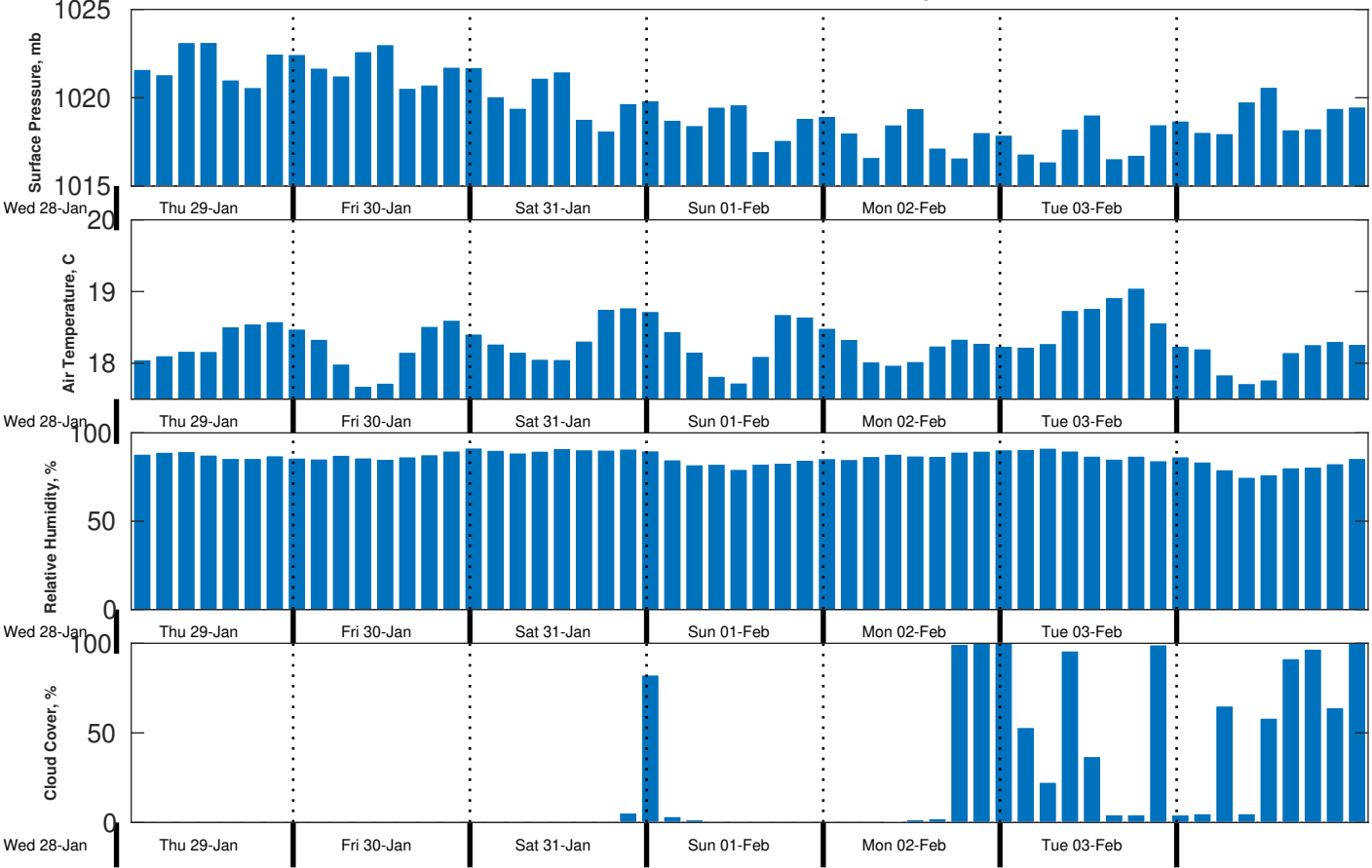
Met Forecast for CSA (ONHYM) PPL EBS - Western Sahara from 29-Jan-2026 00:00:00 to 05-Feb-2026 00:00:00
