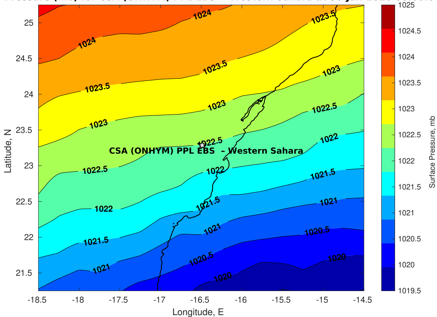
Surface Pressure (mb) for CSA (ONHYM) PPL EBS - Western Sahara at 30-Jan-2026 00:00:00
