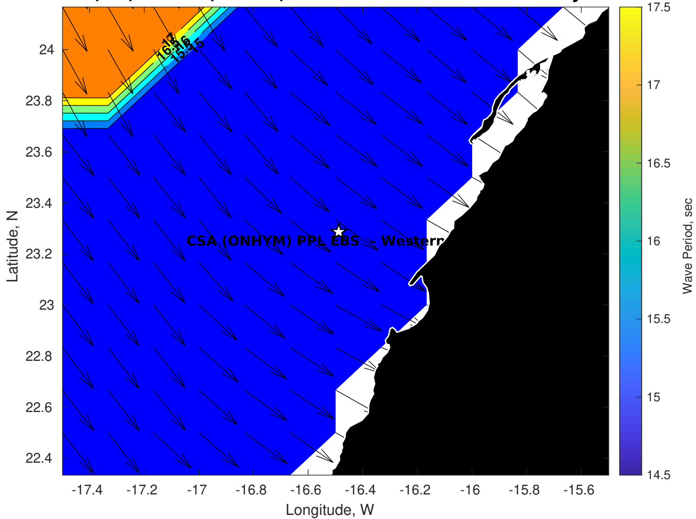
GFS Wave Period (sec) for CSA (ONHYM) PPL EBS - Western Sahara at 29-Jan-2026 09:00:00
