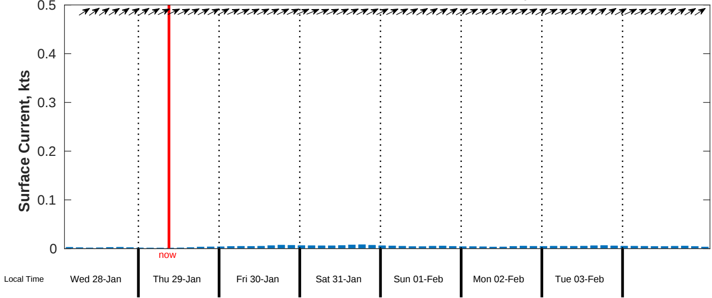
Surface Current Forecast for CSA (ONHYM) PPL EBS - Western Sahara from 28-Jan-2026 00:00:00 to 05-Feb-2026 00:00:00
