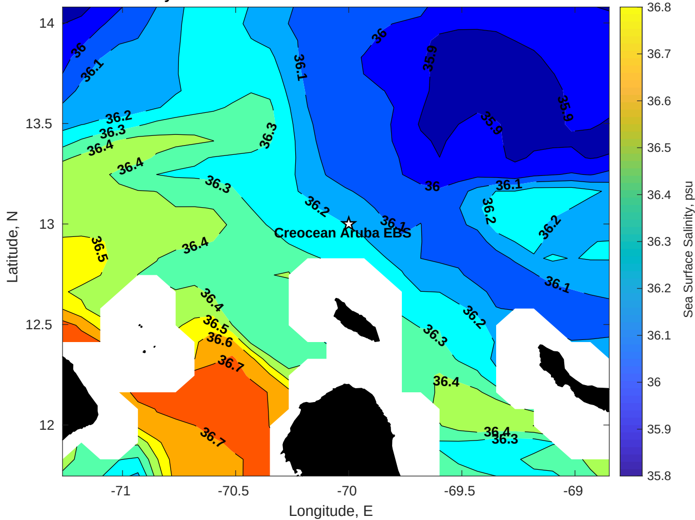
Surface Salinity for Creoccean Aruba EBS at 28-Jan-2026 00:00:00
