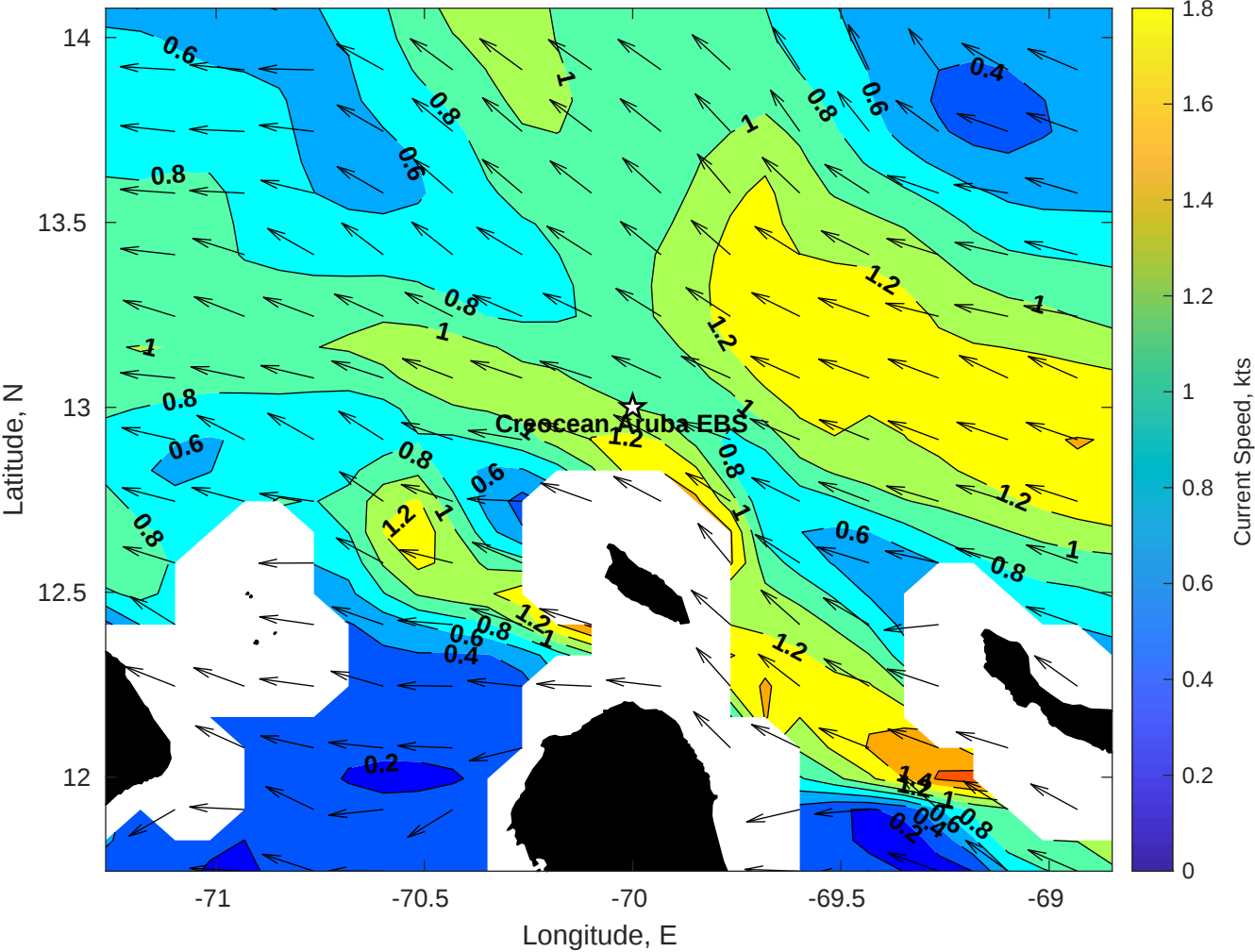
Surface Currents for Creocean Aruba EBS at 28-Jan-2026 00:00:00
