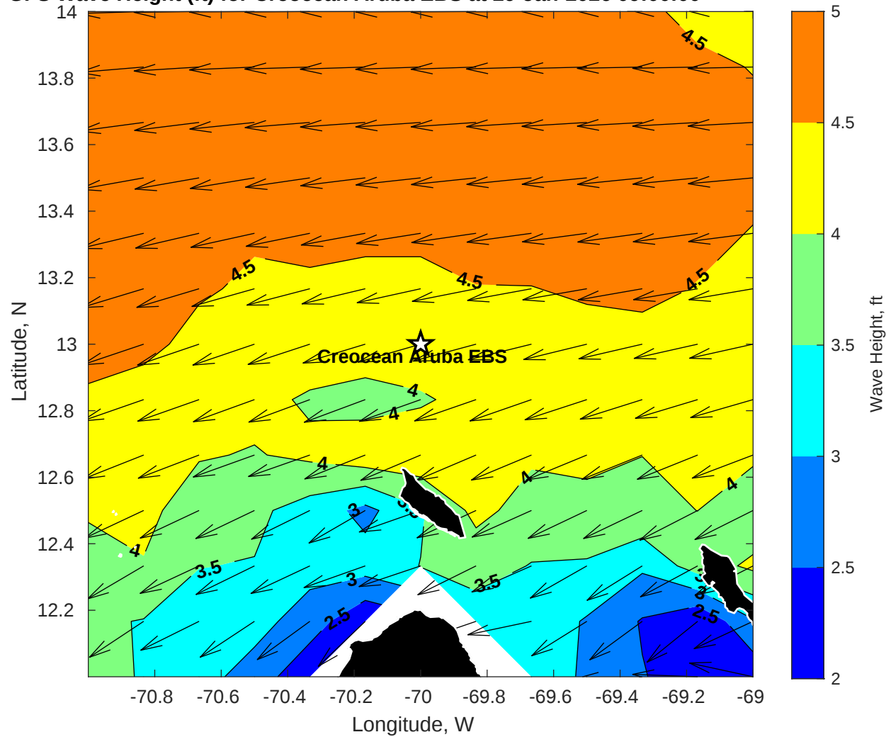
GFS Wave Height (ft) for Creolean Aruba EBS at 29-Jan-2026 09:00:00
