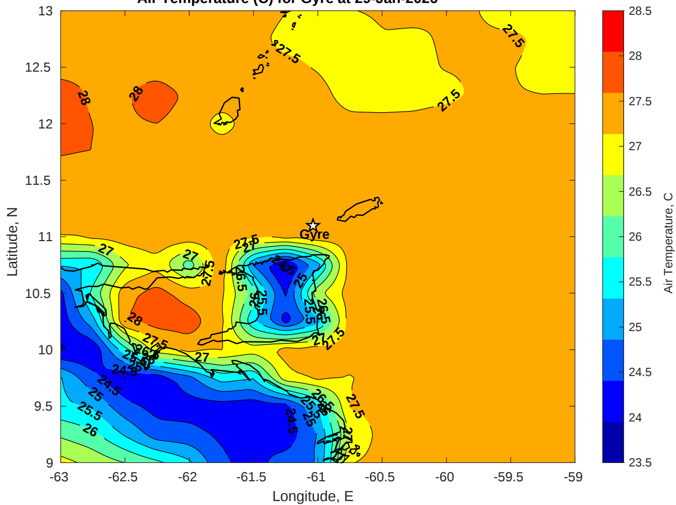
Air Temperature (C) for Gyre at 29-Jan-2026
