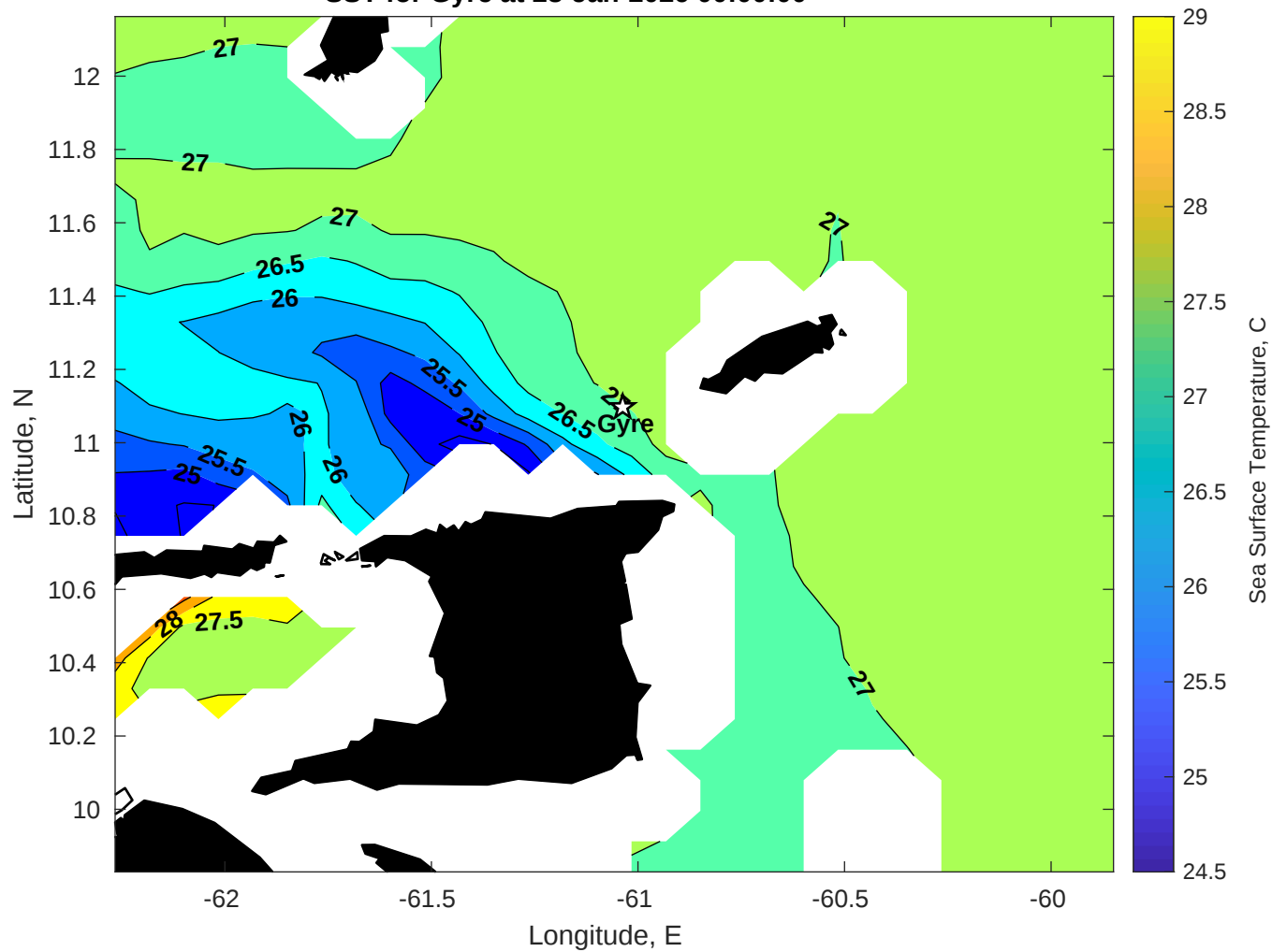
SST for Gyre at 28-Jan-2026 00:00:00
