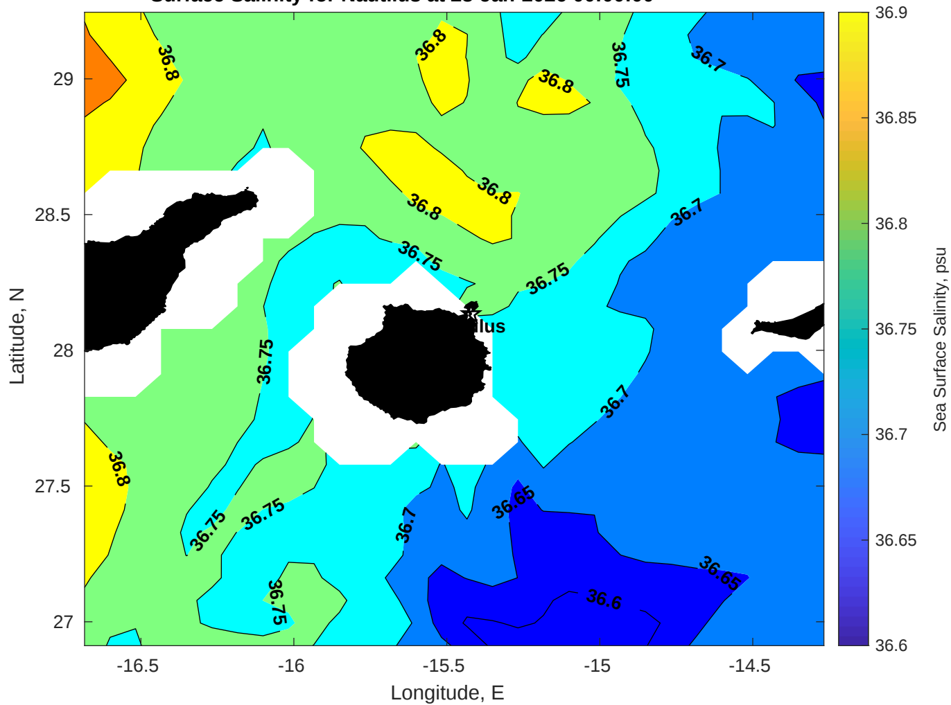
Surface Salinity for Nautilus at 28-Jan-2026 00:00:00
