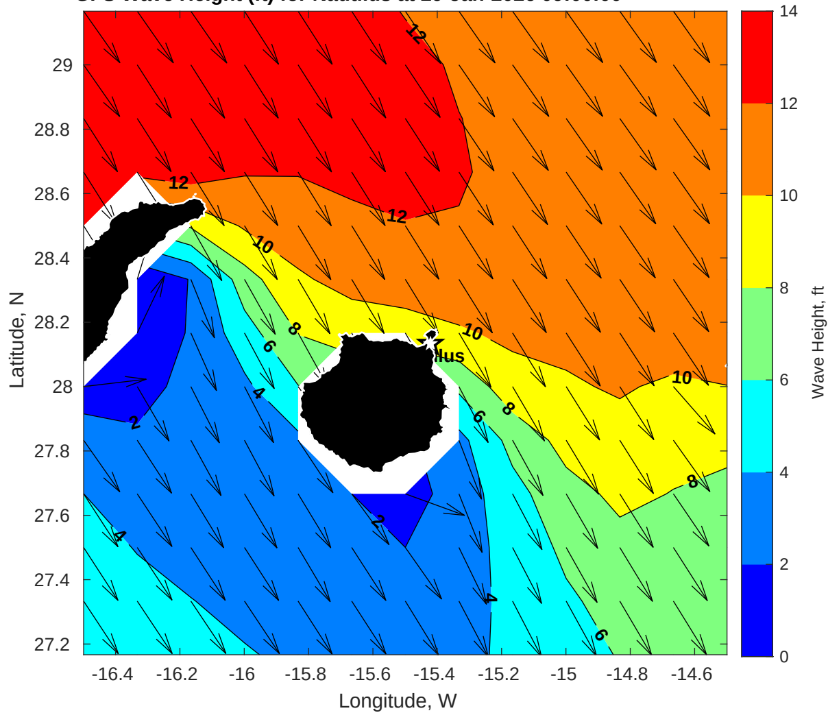
GFS Wave Height (ft) for Nautilus at 29-Jan-2026 09:00:00
