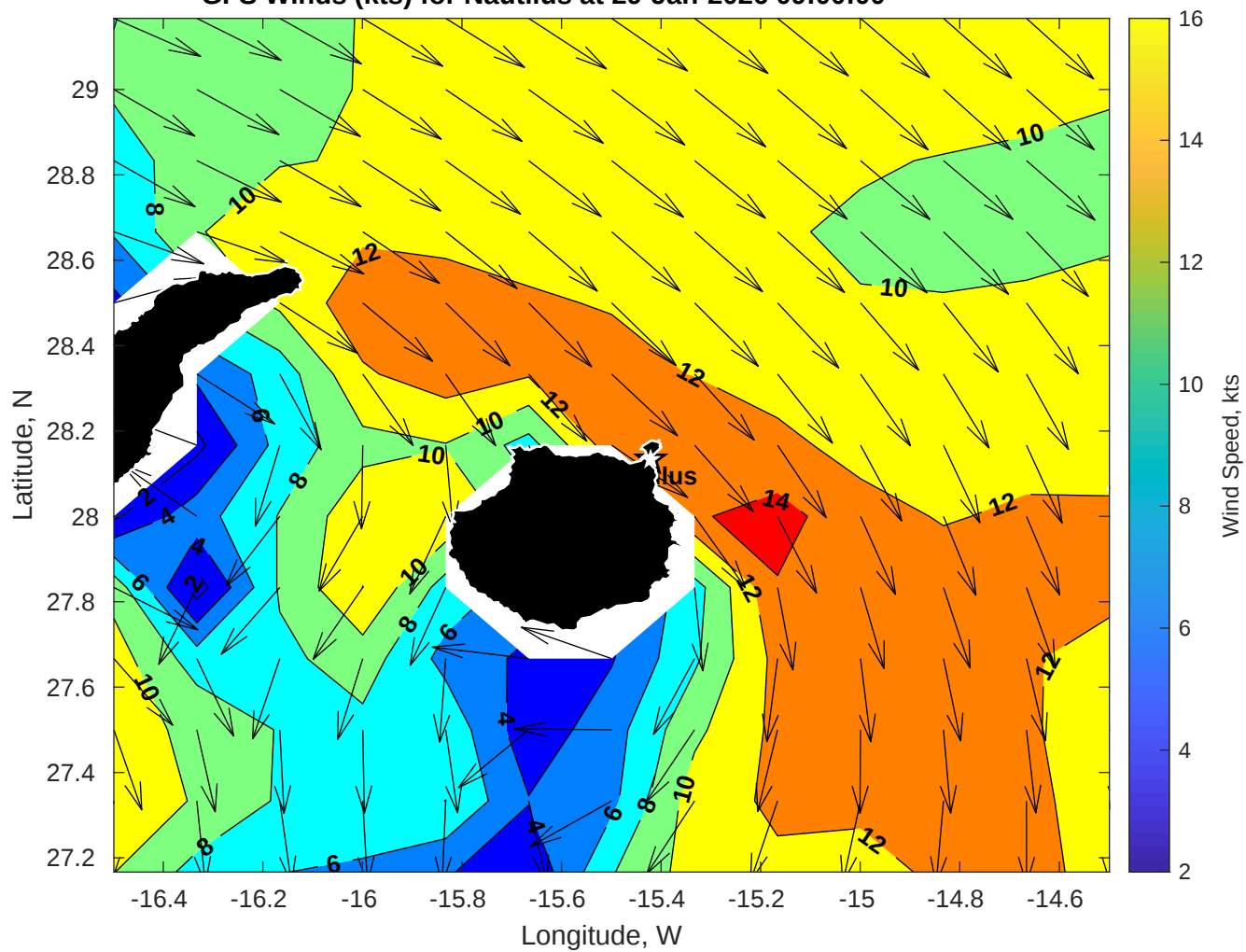
GFS Winds (kts) for Nautilus at 29-Jan-2026 09:00:00
