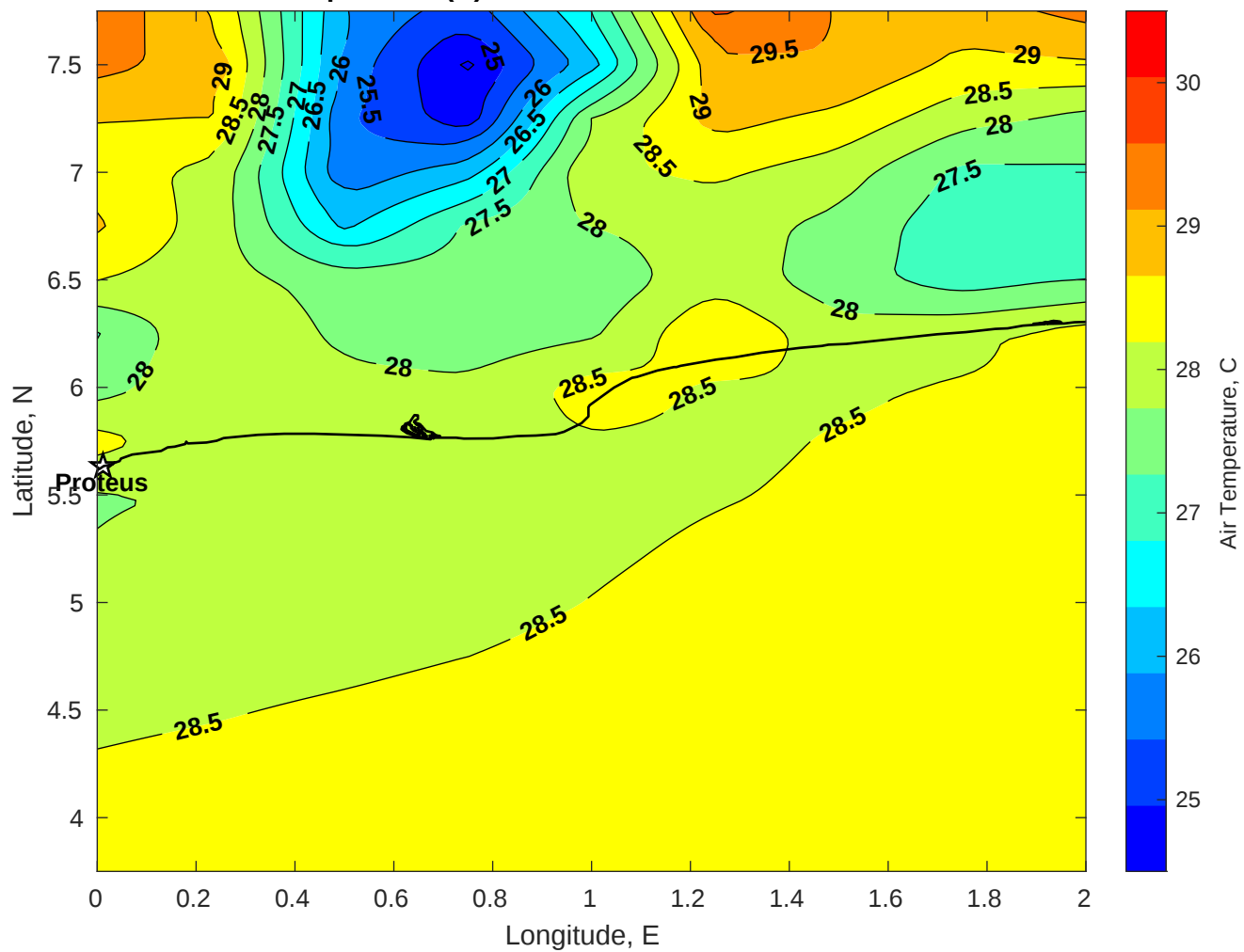
Air Temperature (C) for Proteus at 29-Jan-2026
