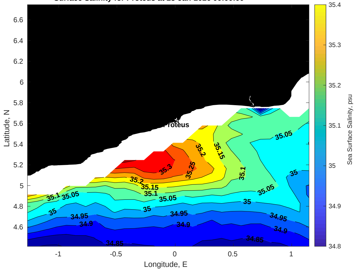
Surface Salinity for Proteus at 28-Jan-2026 00:00:00
