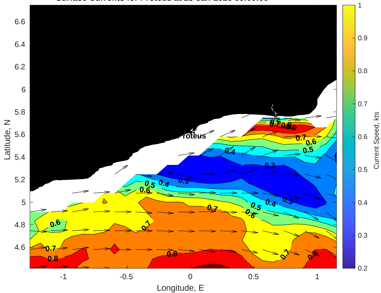
Surface Currents for Proteus at 28-Jan-2026 00:00:00
