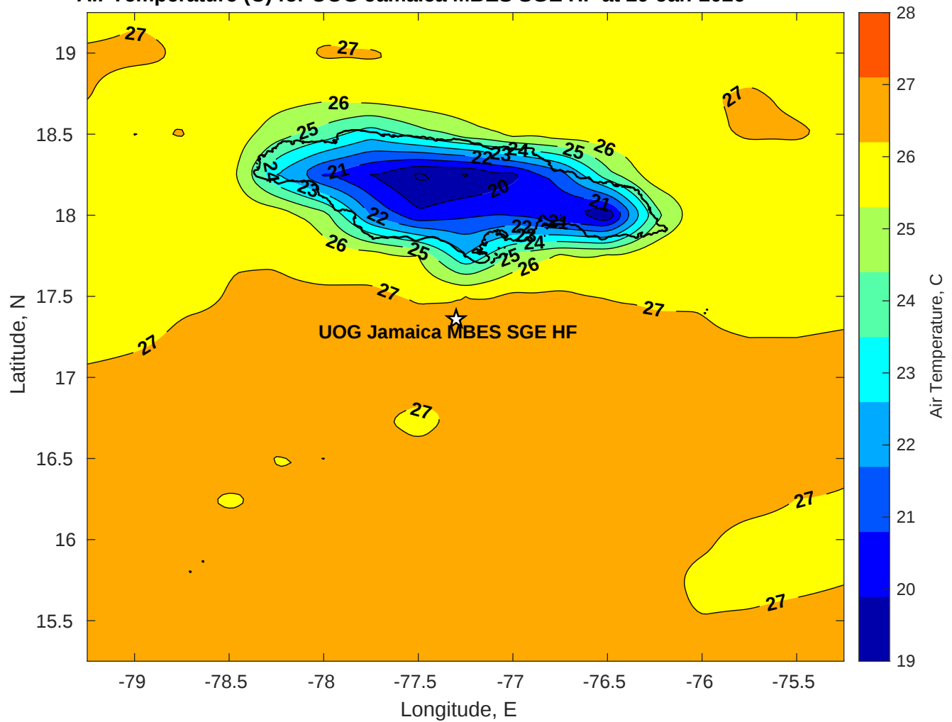
Air Temperature (C) for UOG Jamaica MBES SGE HF at 29-Jan-2026
