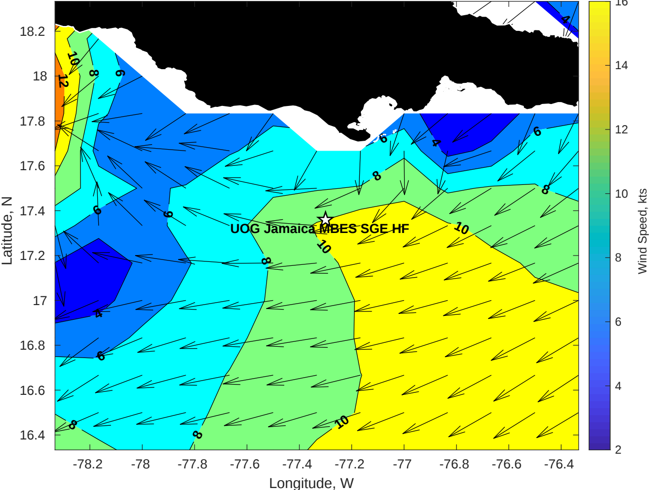
GFS Winds (kts) for UOG Jamaica MBES SGE HF at 29-Jan-2026 09:00:00
