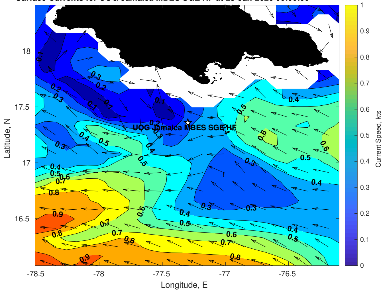
Surface Currents for UOG Jamaica MBES SGE HF at 28-Jan-2026 00:00:00
