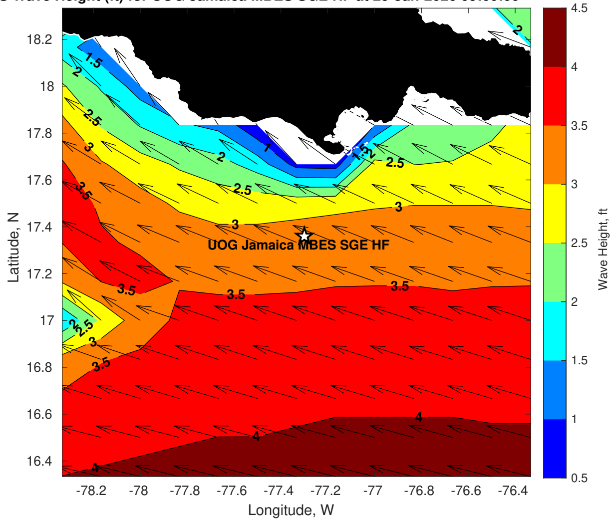
GFS Wave Height (ft) for UOG Jamaica MBES SGE HF at 29-Jan-2026 09:00:00
