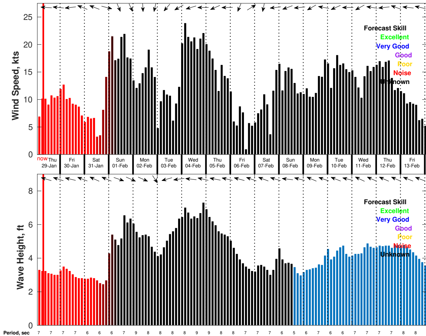
Wind & Wave Forecast for UOG Jamaica MBES SGE HF from 29-Jan-2026 02:00:00 to 14-Feb-2026 02:00:00
