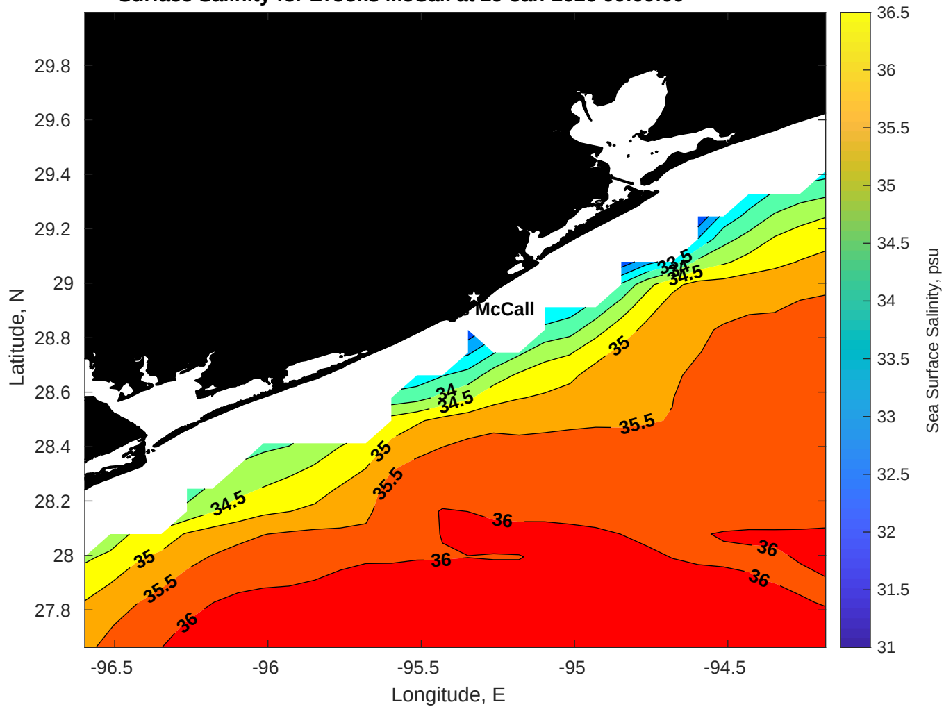
Surface Salinity for Brooks McCall at 29-Jan-2026 00:00:00
