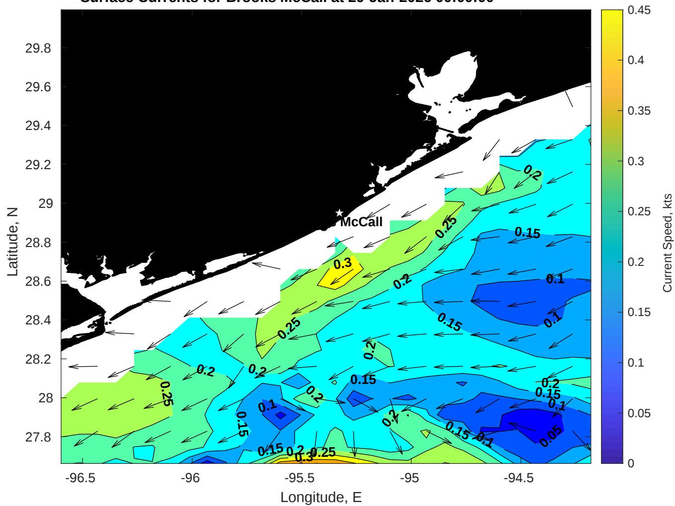
Surface Currents for Brooks McCall at 29-Jan-2026 00:00:00
