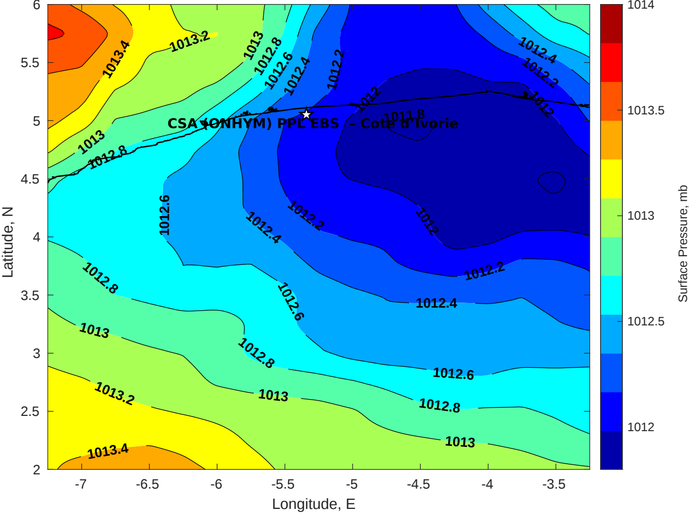
Surface Pressure (mb) for CSA (ONHYM) PPL EBS - Cote d'Ivoire at 30-Jan-2026 00:00:00
