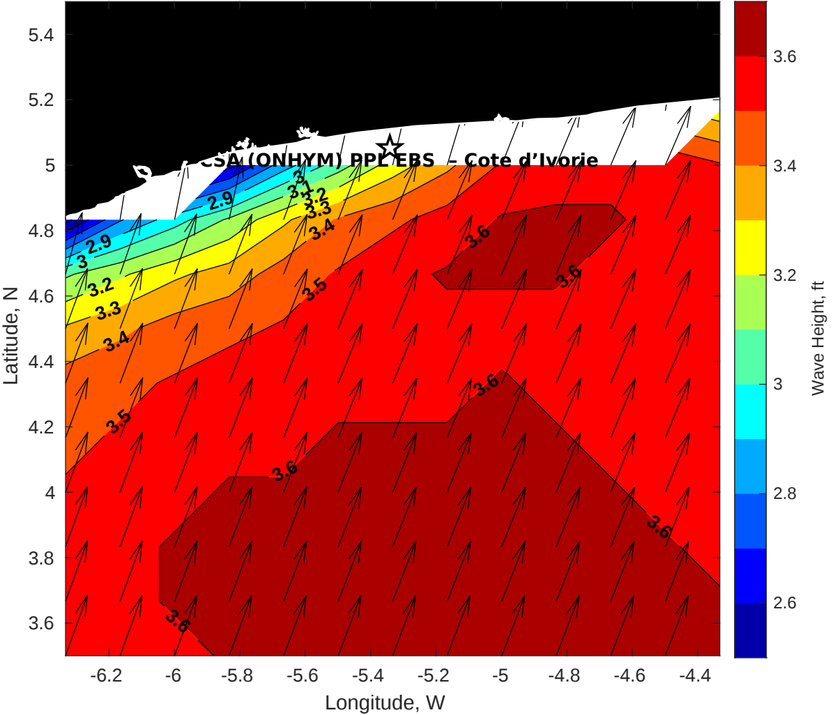
GFS Wave Height (ft) for CSA (ONHYM) PPL EBS - Cote d'Ivoire at 30-Jan-2026 09:00:00
