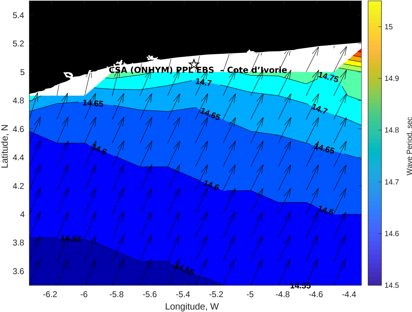
GFS Wave Period (sec) for CSA (ONHYM) PPL EBS - Cote d'Ivoire at 30-Jan-2026 09:00:00
