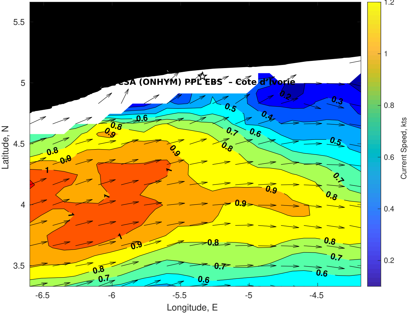
Surface Currents for CSA (ONHYM) PPL EBS - Cote d'Ivoire at 29-Jan-2026 00:00:00
