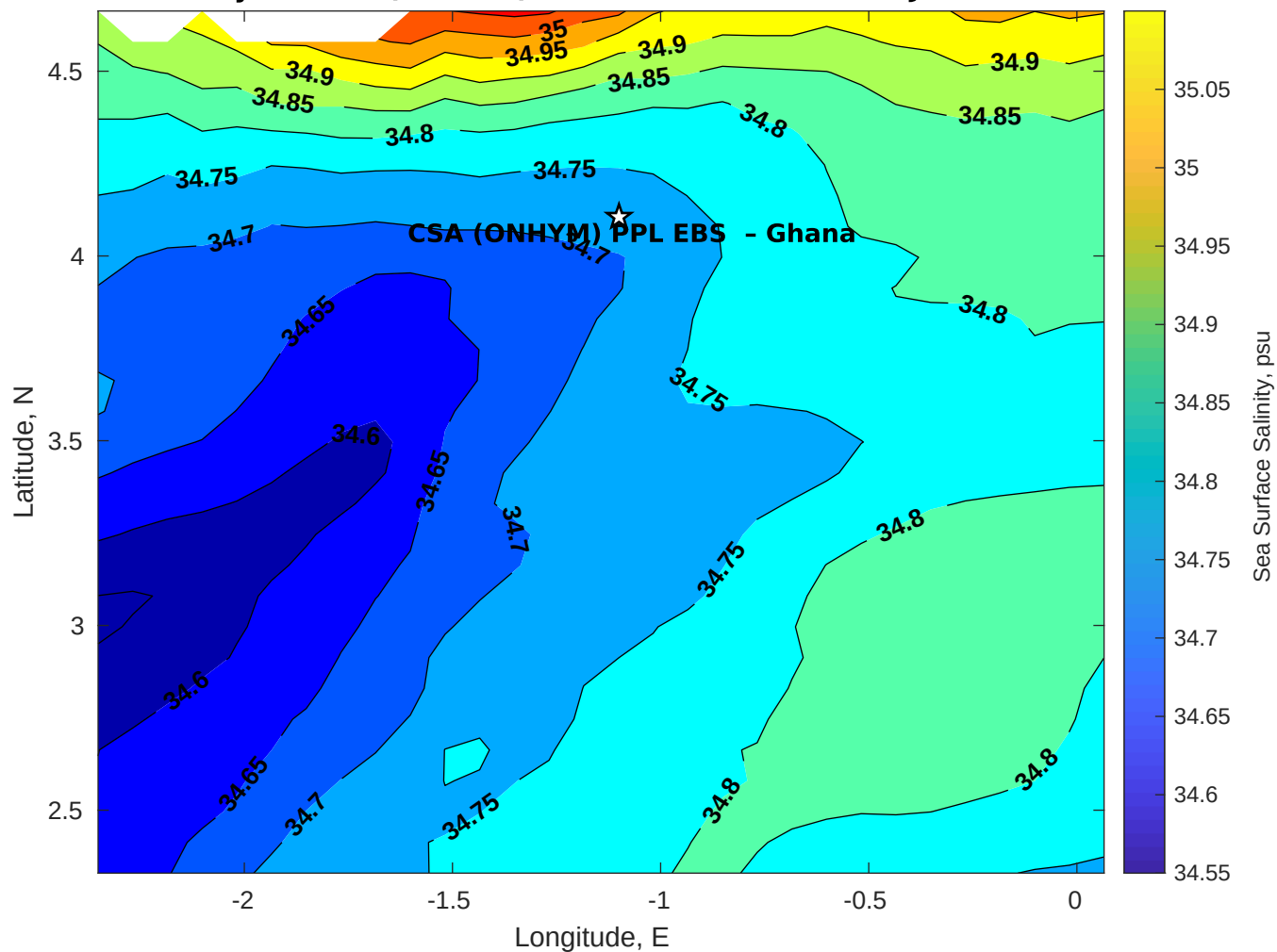
Surface Salinity for CSA (ONHYM) PPL EBS - Ghana at 29-Jan-2026 00:00:00
