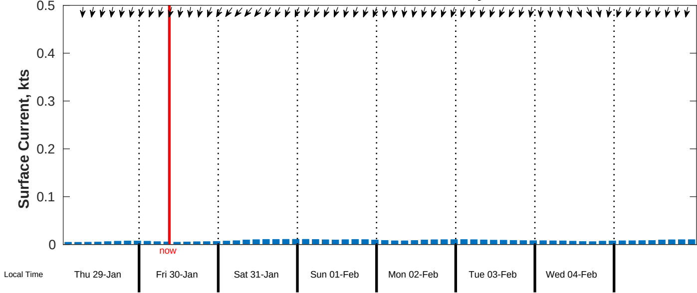
Surface Current Forecast for CSA (ONHYM) PPL EBS - Ghana from 29-Jan-2026 00:00:00 to 06-Feb-2026 00:00:00
