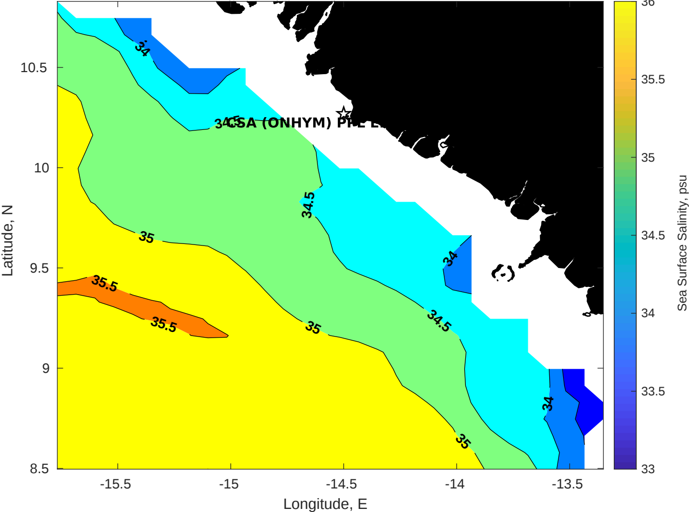
Surface Salinity for CSA (ONHYM) PPL EBS - Guinea at 29-Jan-2026 00:00:00
