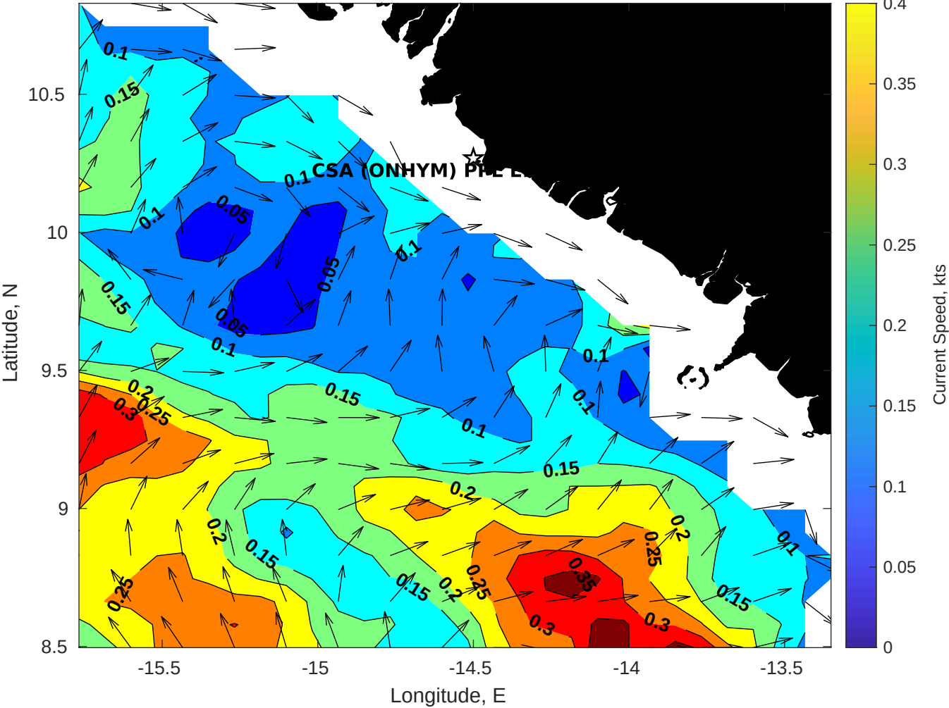
Surface Currents for CSA (ONHYM) PPL EBS - Guinea at 29-Jan-2026 00:00:00
