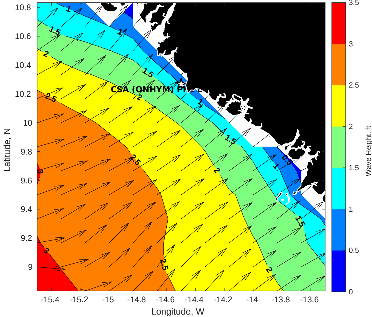
GFS Wave Height (ft) for CSA (ONHYM) PPL EBS - Guinea at 30-Jan-2026 09:00:00
