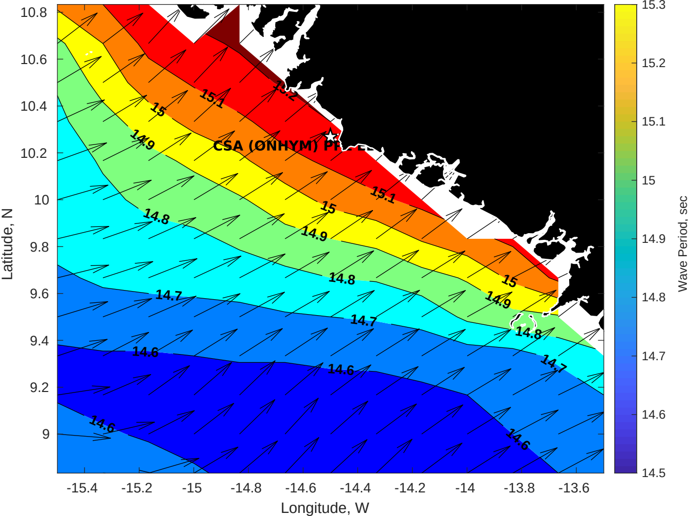
GFS Wave Period (sec) for CSA (ONHYM) PPL EBS - Guinea at 30-Jan-2026 09:00:00
