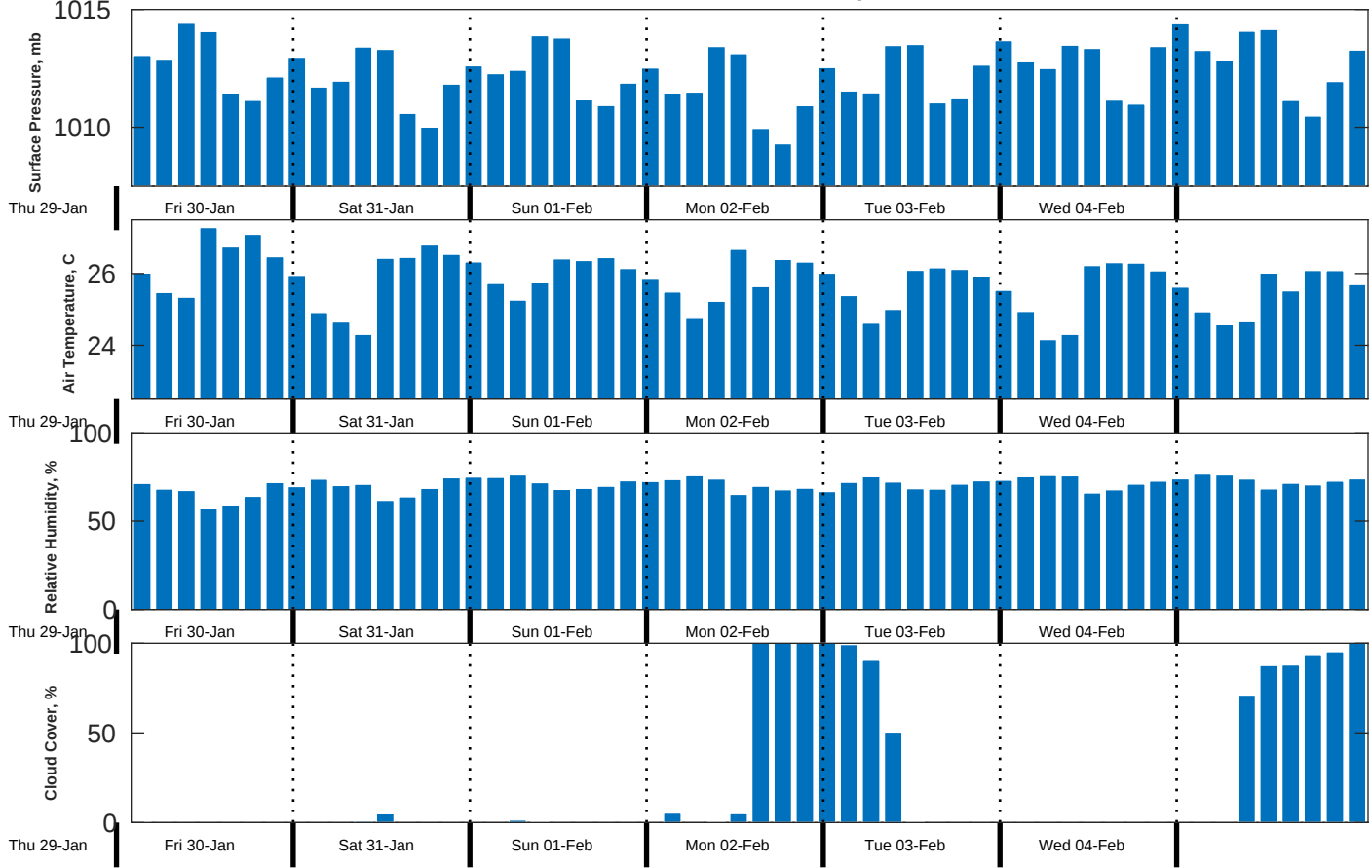
Met Forecast for CSA (ONHYM) PPL EBS - Guinea from 30-Jan-2026 00:00:00 to 06-Feb-2026 00:00:00
