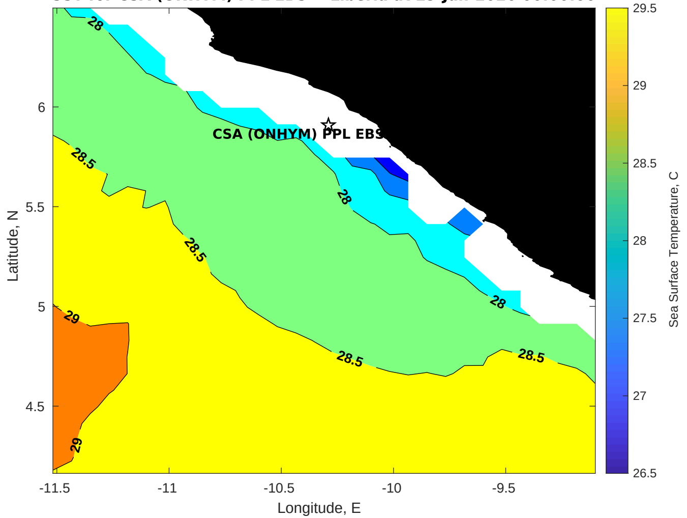
SST for CSA (ONHYM) PPL EBS - Liberia at 29-Jan-2026 00:00:00
