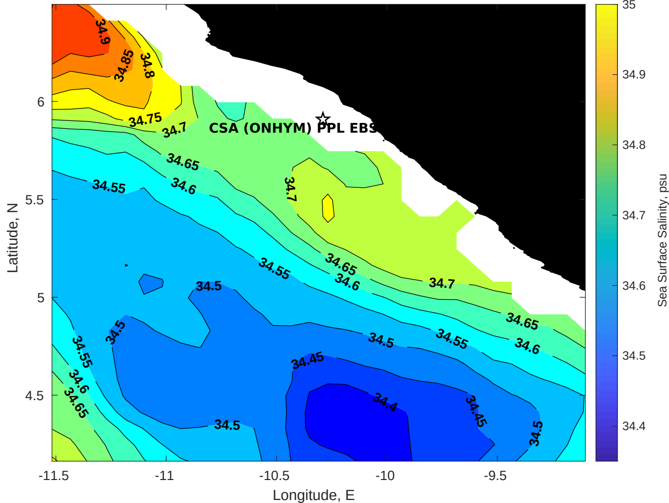
Surface Salinity for CSA (ONHYM) PPL EBS - Liberia at 29-Jan-2026 00:00:00
