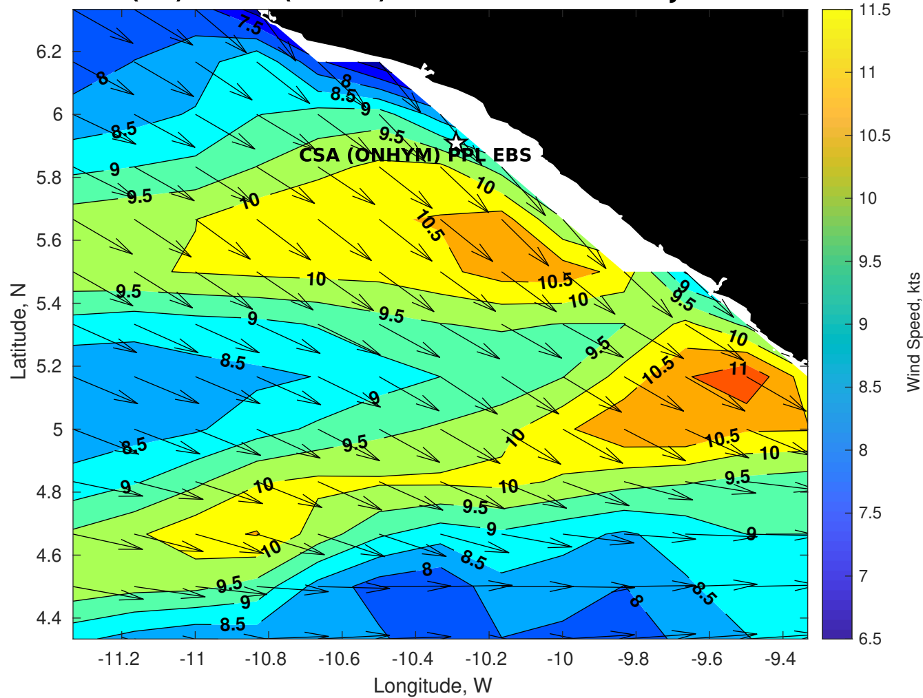
GFS Winds (kts) for CSA (ONHYM) PPL EBS - Liberia at 30-Jan-2026 09:00:00
