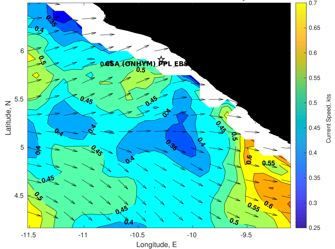
Surface Currents for CSA (ONHYM) PPL EBS - Liberia at 29-Jan-2026 00:00:00
