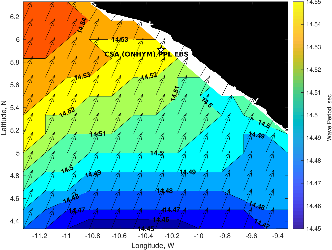
GFS Wave Period (sec) for CSA (ONHYM) PPL EBS - Liberia at 30-Jan-2026 09:00:00
