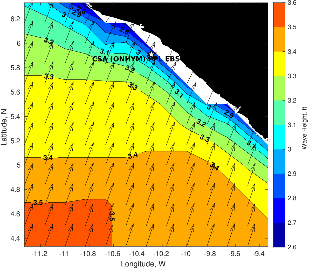
GFS Wave Height (ft) for CSA (ONHYM) PPL EBS - Liberia at 30-Jan-2026 09:00:00
