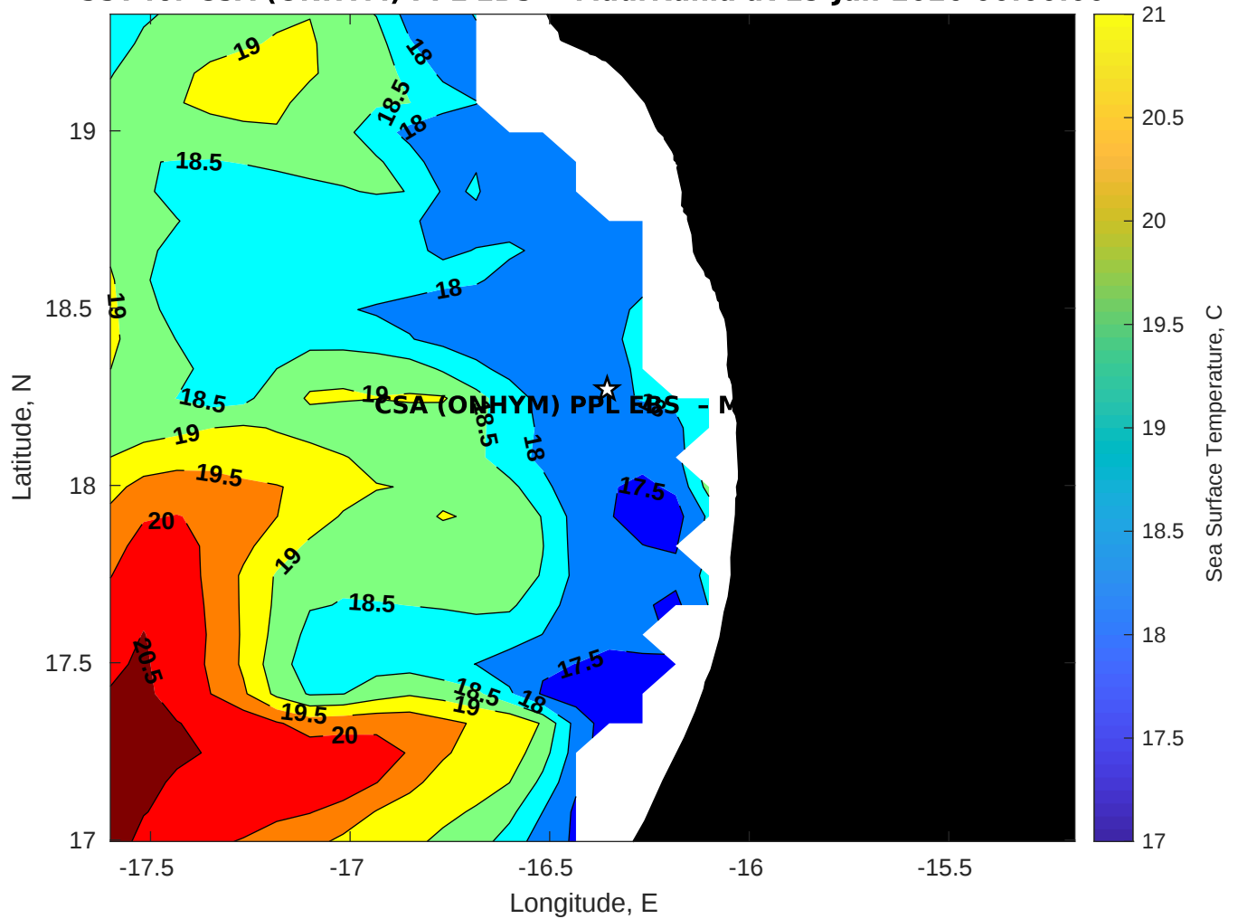
SST for CSA (ONHYM) PPL EBS - Mauritania at 29-Jan-2026 00:00:00
