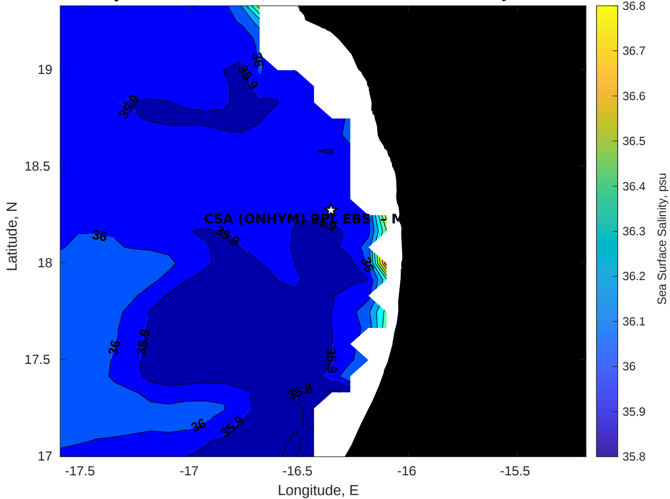
Surface Salinity for CSA (ONHYM) PPL EBS - Mauritania at 29-Jan-2026 00:00:00
