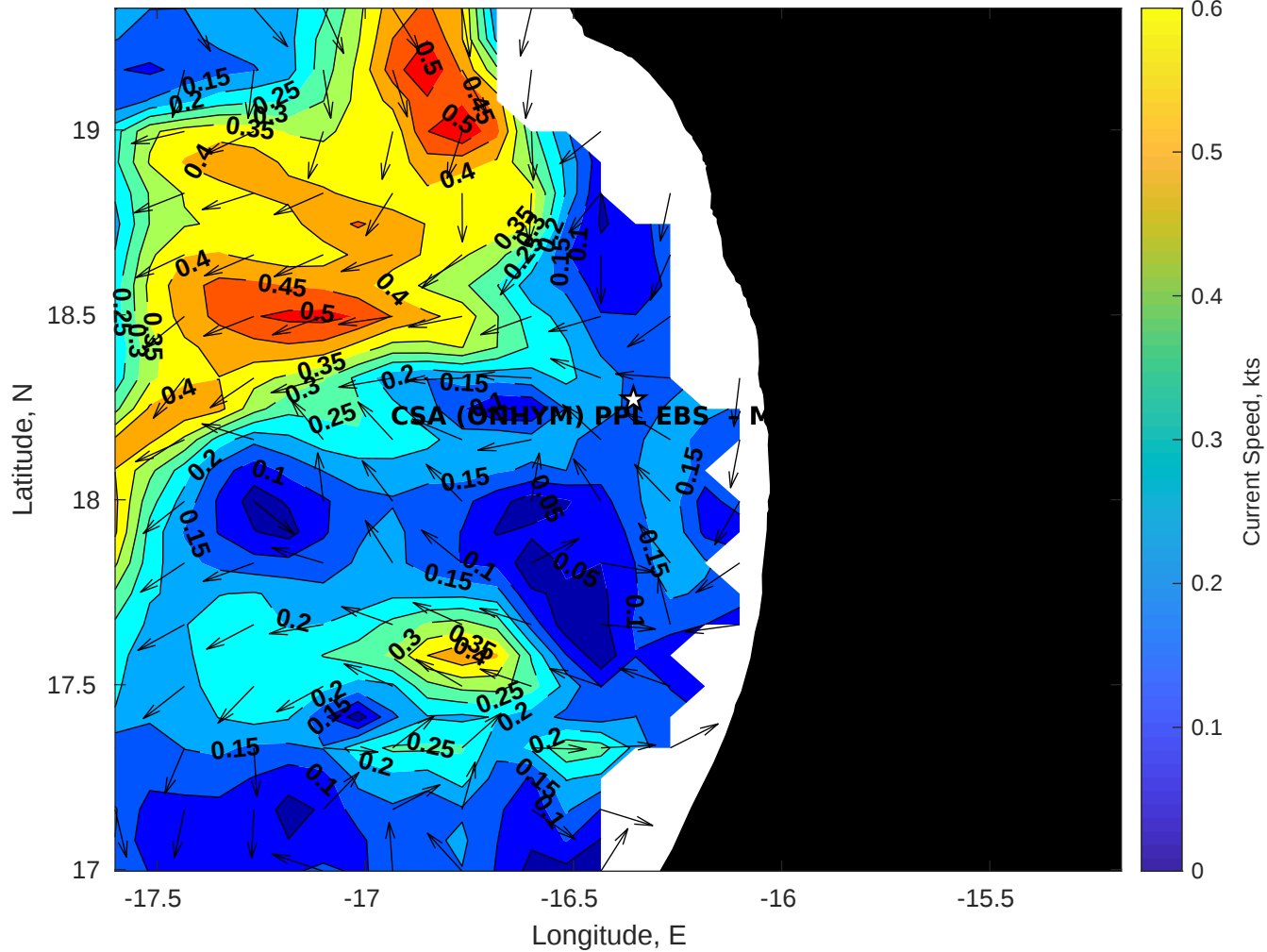
Surface Currents for CSA (ONHYM) PPL EBS - Mauritania at 29-Jan-2026 00:00:00
