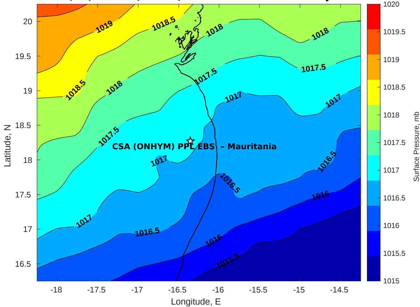
Surface Pressure (mb) for CSA (ONHYM) PPL EBS - Mauritania at 31-Jan-2026 00:00:00
