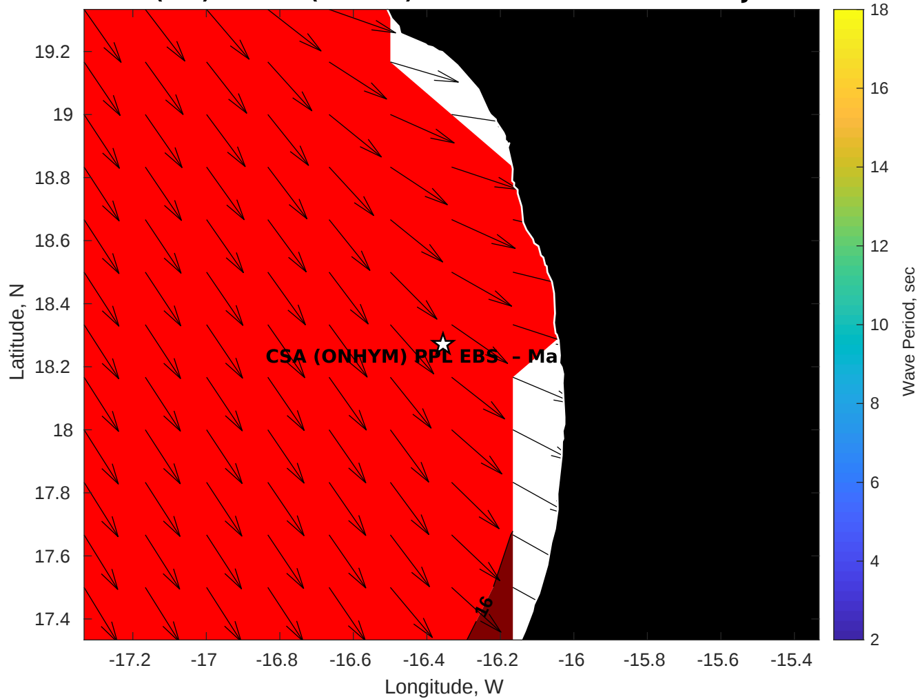
GFS Wave Period (sec) for CSA (ONHYM) PPL EBS - Mauritania at 30-Jan-2026 09:00:00
