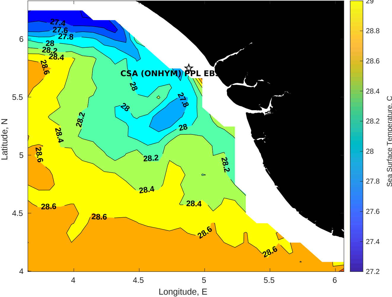
SST for CSA (ONHYM) PPL EBS - Nigeria at 29-Jan-2026 00:00:00
