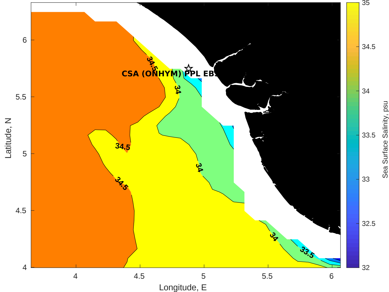
Surface Salinity for CSA (ONHYM) PPL EBS - Nigeria at 29-Jan-2026 00:00:00
