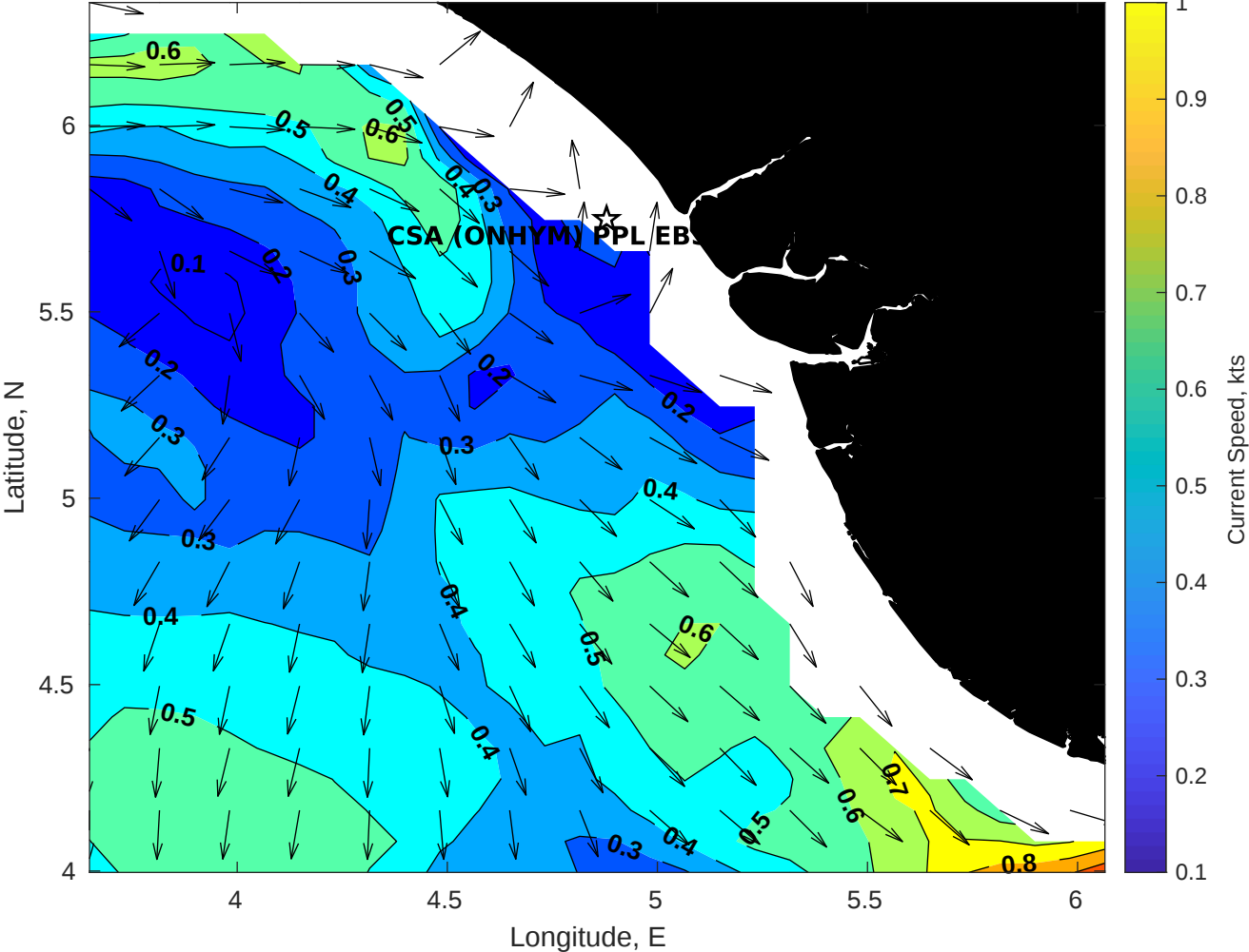
Surface Currents for CSA (ONHYM) PPL EBS - Nigeria at 29-Jan-2026 00:00:00
