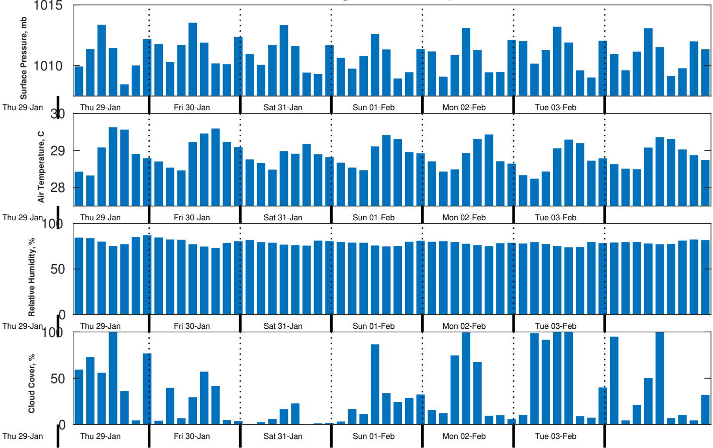
Met Forecast for CSA (ONHYM) PPL EBS - Nigeria from 30-Jan-2026 00:00:00 to 06-Feb-2026 00:00:00
