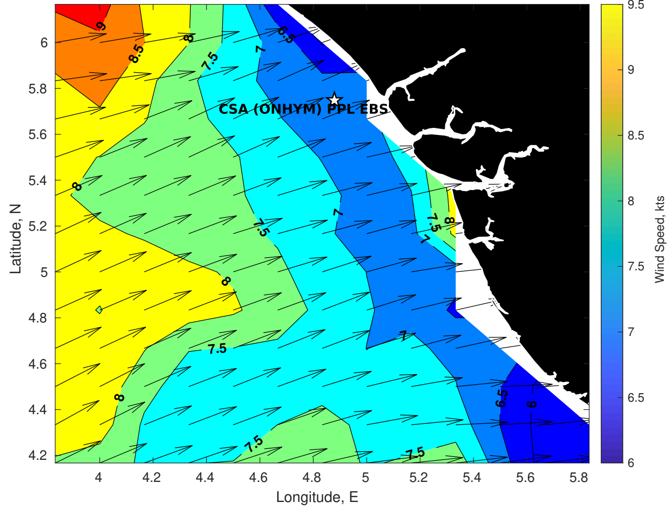
GFS Winds (kts) for CSA (ONHYM) PPL EBS - Nigeria at 30-Jan-2026 09:00:00
