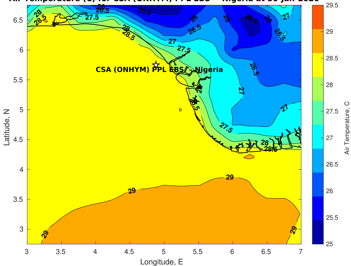
Air Temperature (C) for CSA (ONHYM) PPL EBS - Nigeria at 30-Jan-2026
