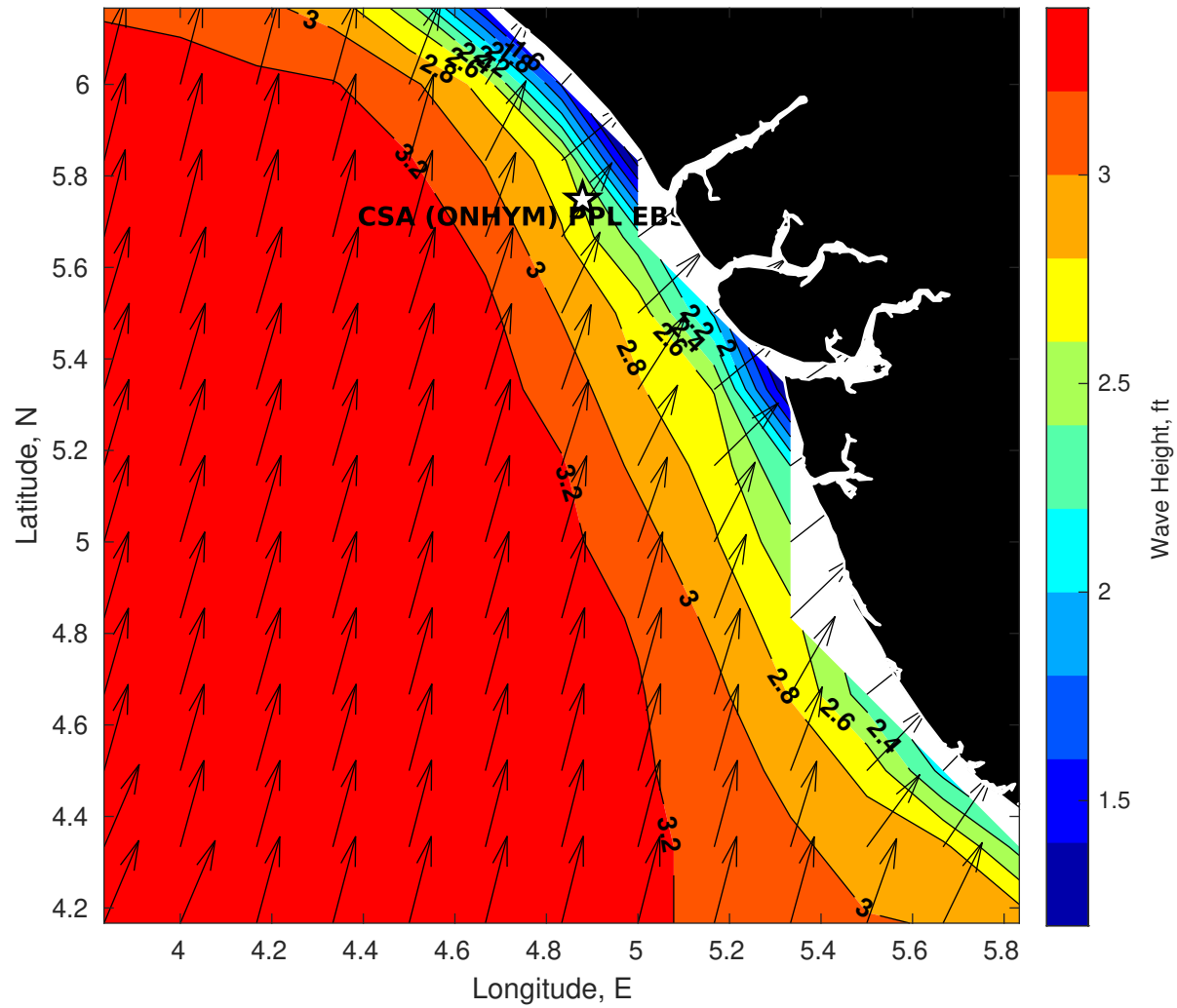
GFS Wave Height (ft) for CSA (ONHYM) PPL EBS - Nigeria at 30-Jan-2026 09:00:00
