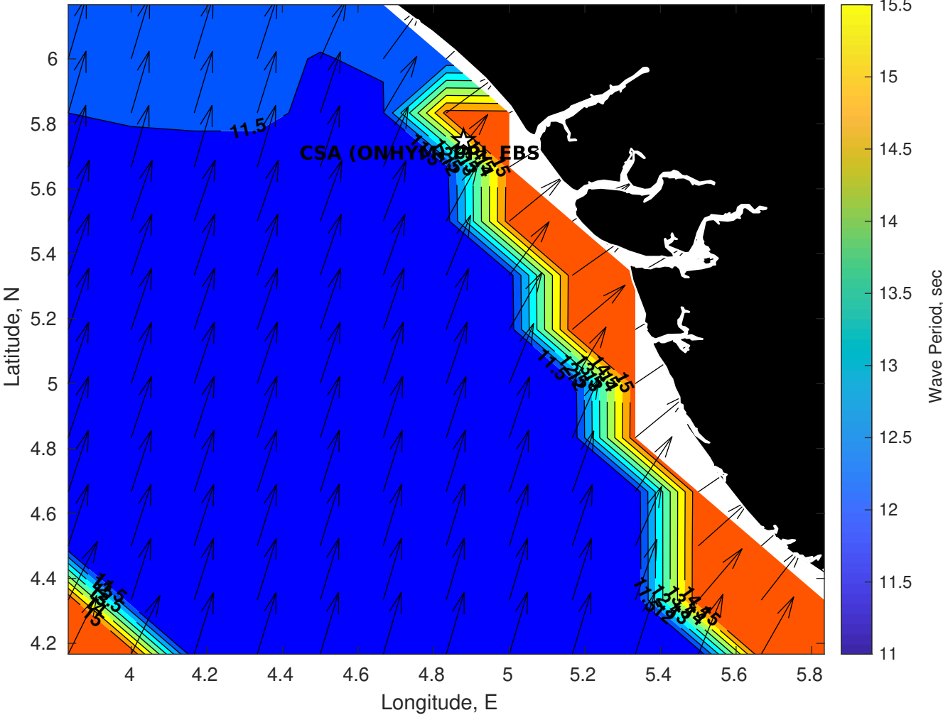
GFS Wave Period (sec) for CSA (ONHYM) PPL EBS - Nigeria at 30-Jan-2026 09:00:00
