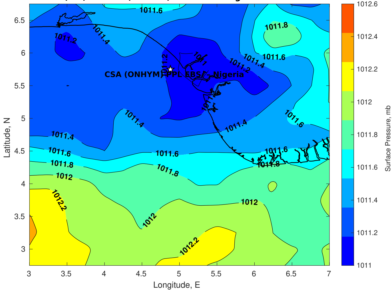
Surface Pressure (mb) for CSA (ONHYM) PPL EBS - Nigeria at 01-Feb-2026 00:00:00
