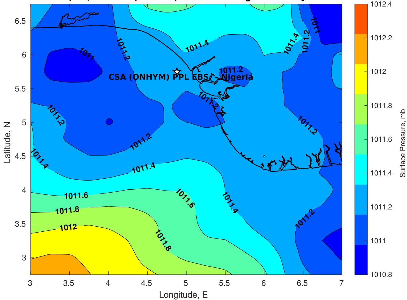
Surface Pressure (mb) for CSA (ONHYM) PPL EBS - Nigeria at 30-Jan-2026 00:00:00
