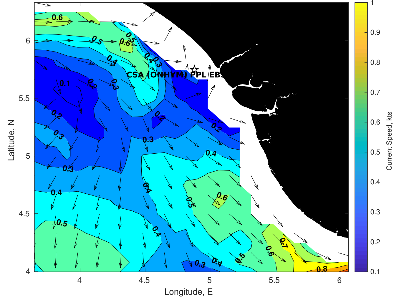
Surface Currents for CSA (ONHYM) PPL EBS - Nigeria at 29-Jan-2026 00:00:00
