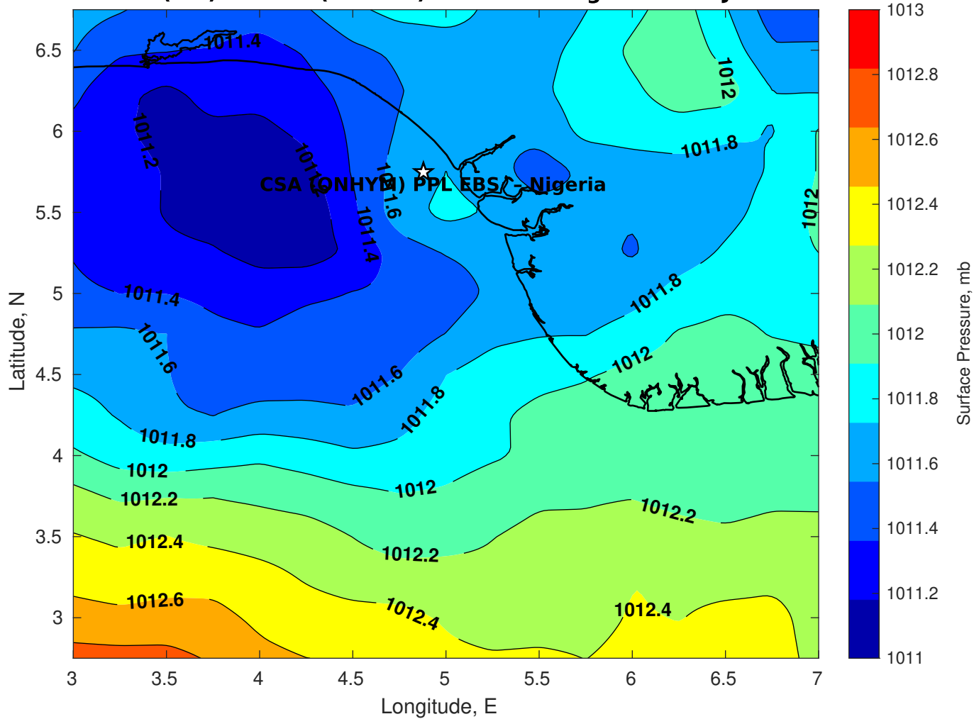
Surface Pressure (mb) for CSA (ONHYM) PPL EBS - Nigeria at 31-Jan-2026 00:00:00
