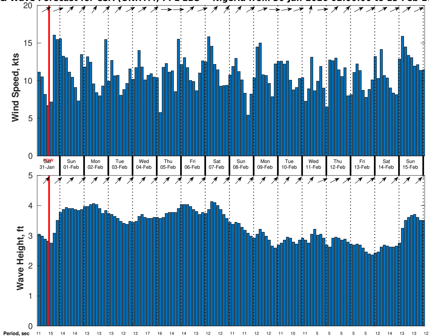
Wind & Wave Forecast for CSA (ONHYM) PPL EBS - Nigeria from 30-Jan-2026 02:00:00 to 15-Feb-2026 02:00:00
