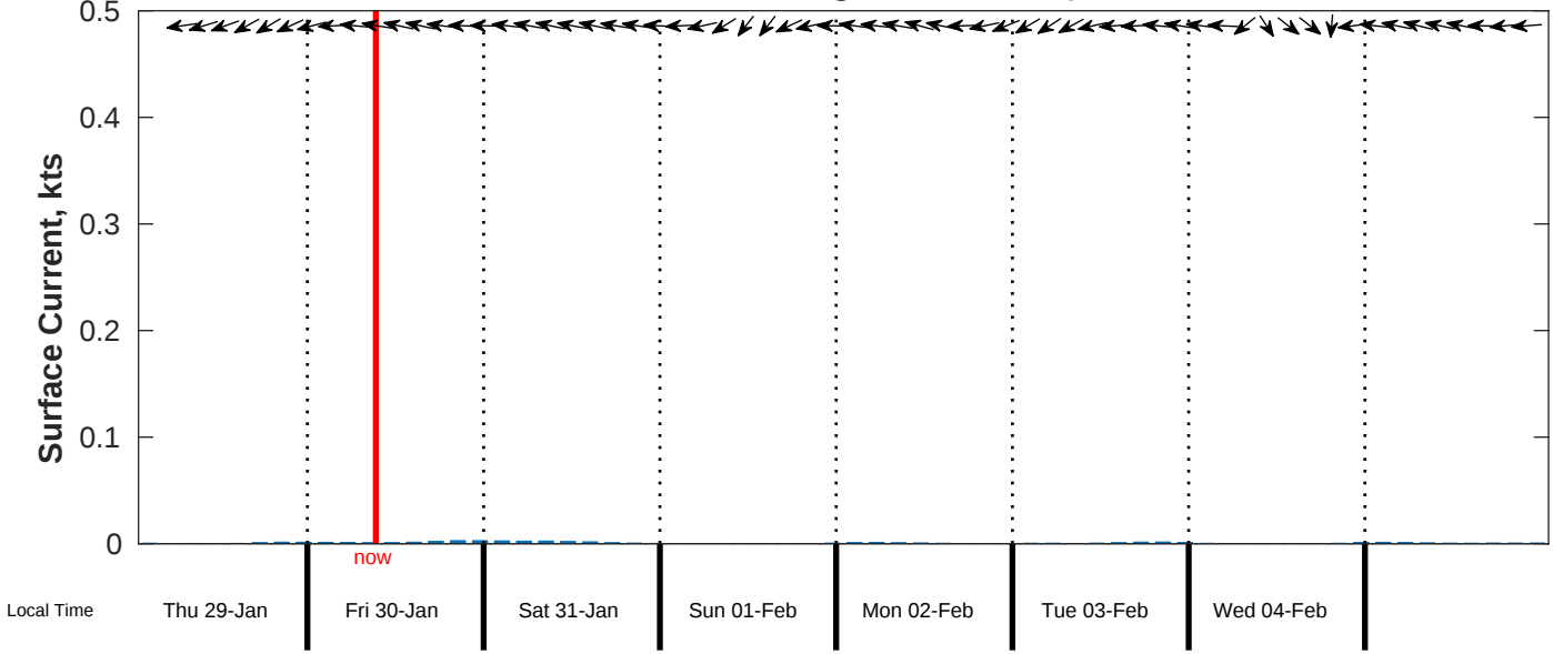
Surface Current Forecast for CSA (ONHYM) PPL EBS - Nigeria from 29-Jan-2026 00:00:00 to 06-Feb-2026 00:00:00
