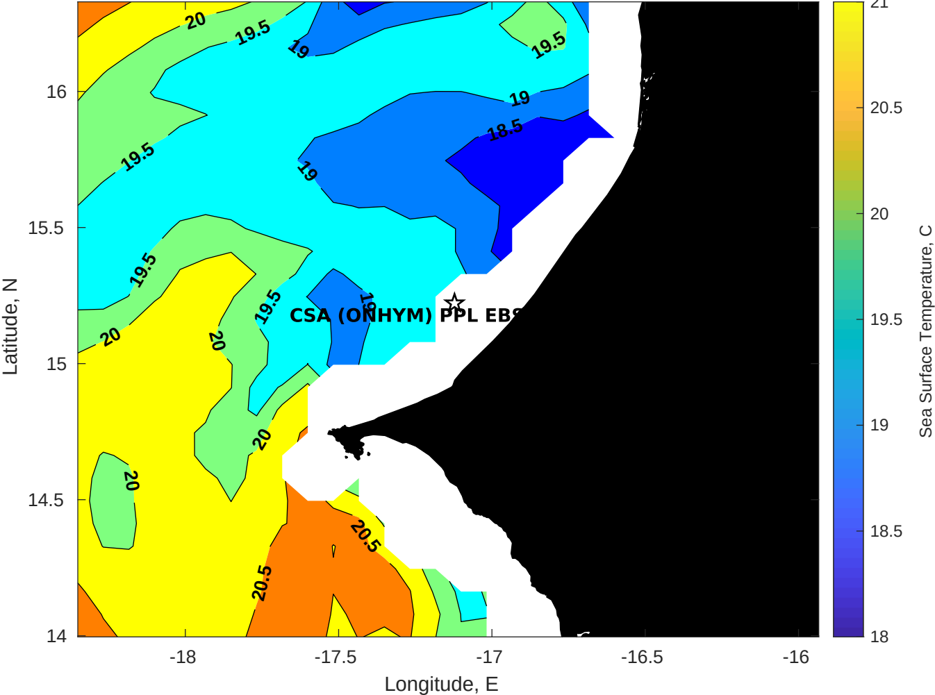
SST for CSA (ONHYM) PPL EBS - Senegal at 29-Jan-2026 00:00:00
