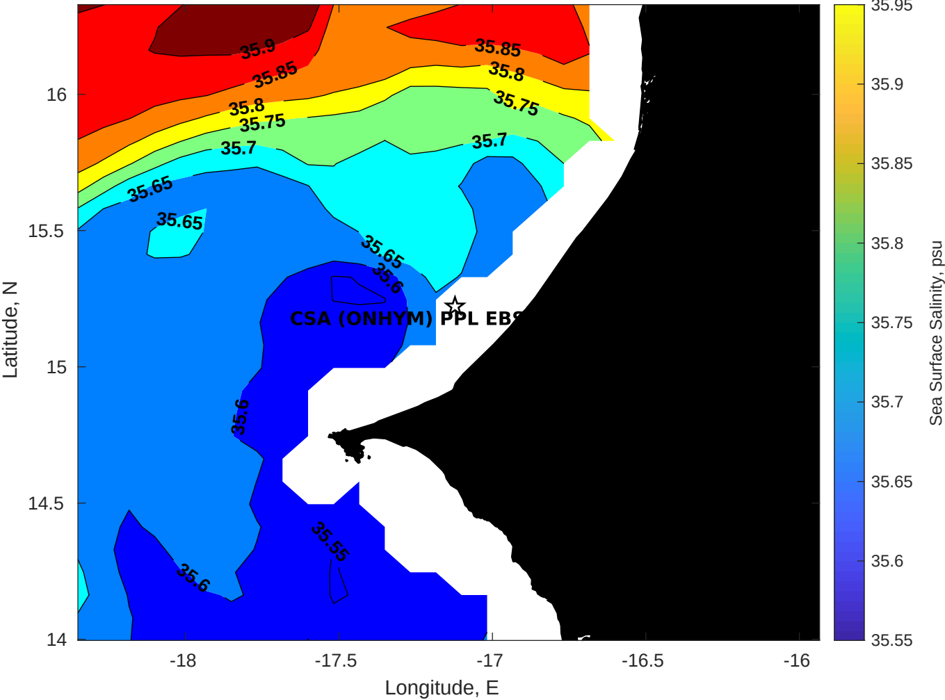
Surface Salinity for CSA (ONHYM) PPL EBS - Senegal at 29-Jan-2026 00:00:00
