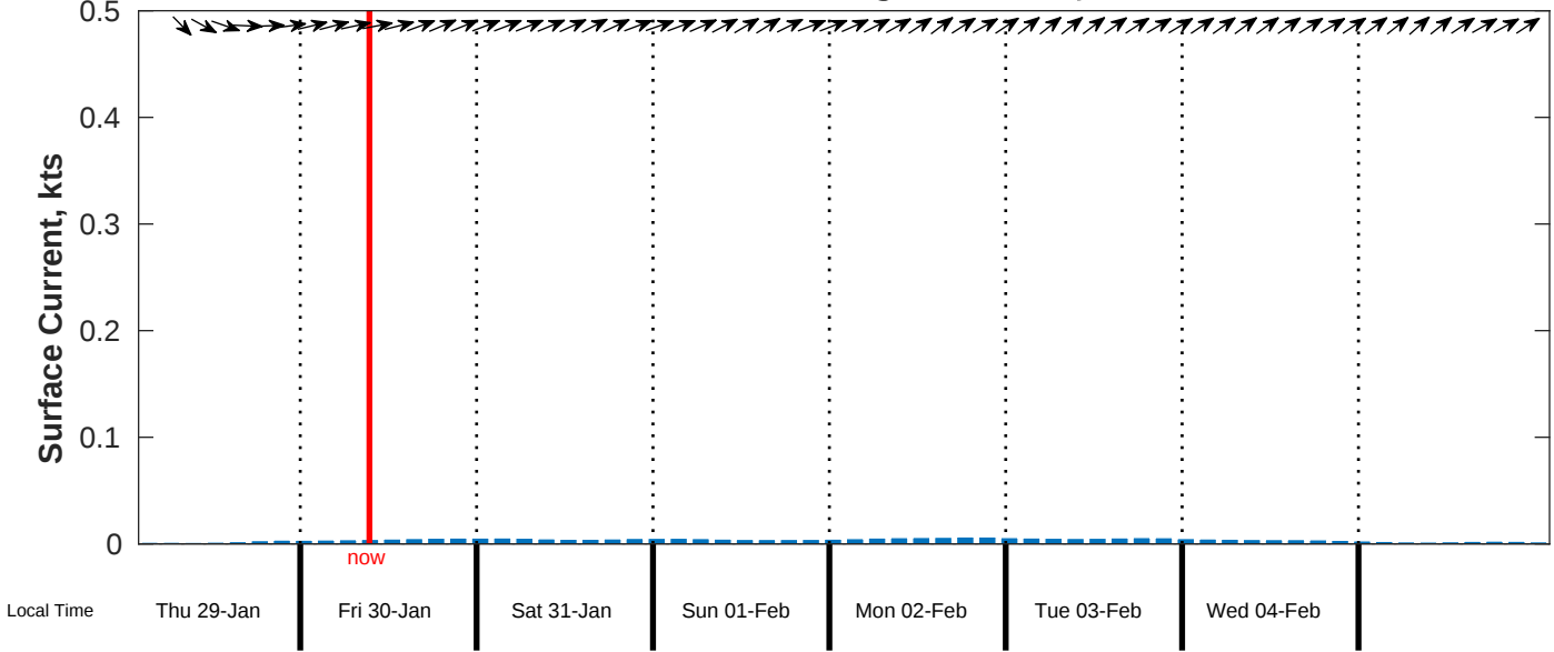
Surface Current Forecast for CSA (ONHYM) PPL EBS - Senegal from 29-Jan-2026 00:00:00 to 06-Feb-2026 00:00:00
