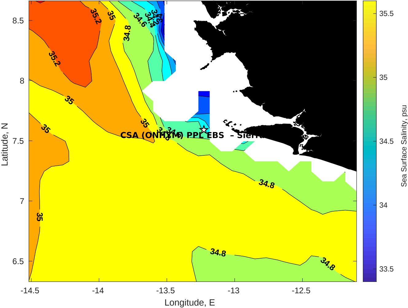
Surface Salinity for CSA (ONHYM) PPL EBS - Sierra Leone at 29-Jan-2026 00:00:00
