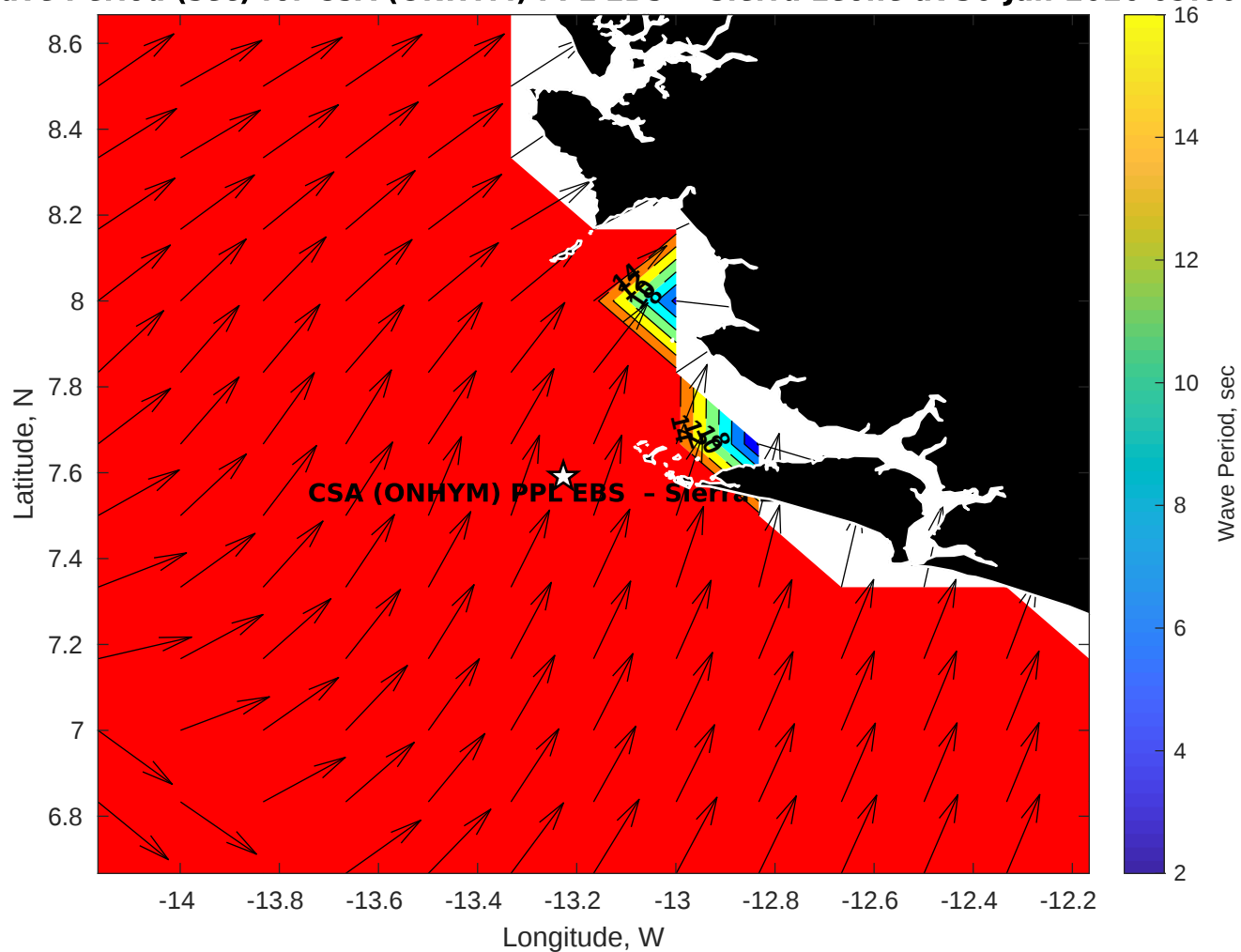
GFS Wave Period (sec) for CSA (ONHYM) PPL EBS - Sierra Leone at 30-Jan-2026 09:00:00
